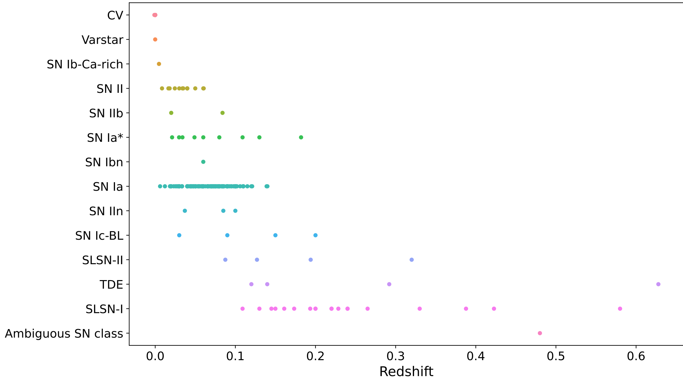
Redshift vs transient class
