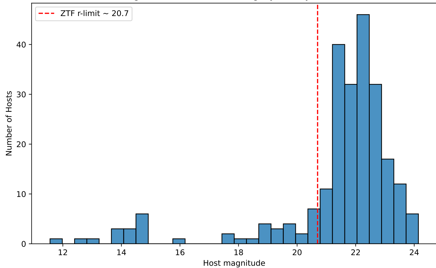
Host Magnitude Distribution — Legacy Survey DECaLS DR9
