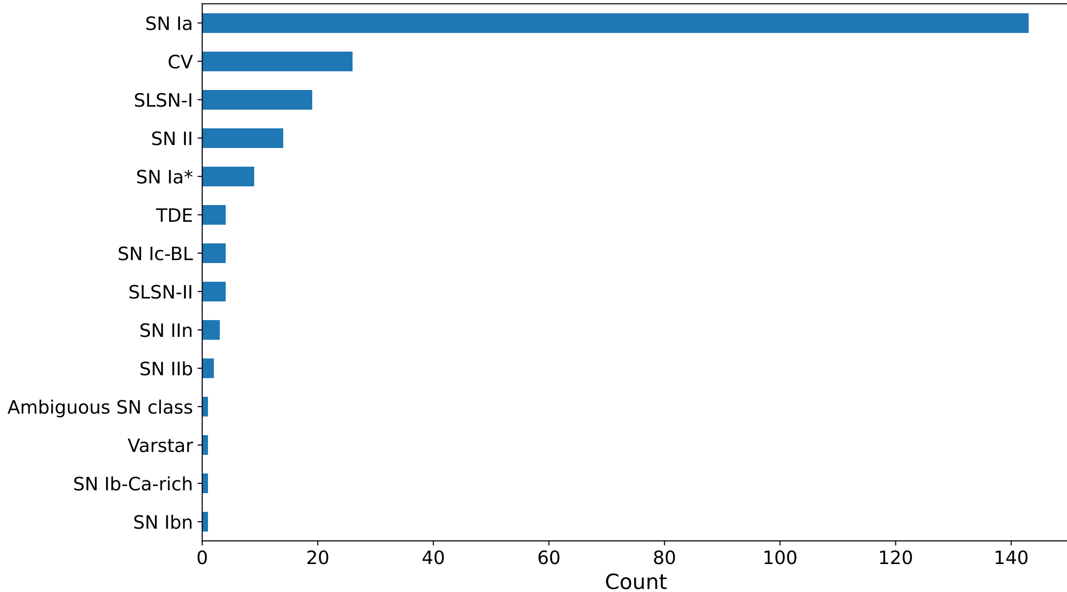
Distribution of transient classes
