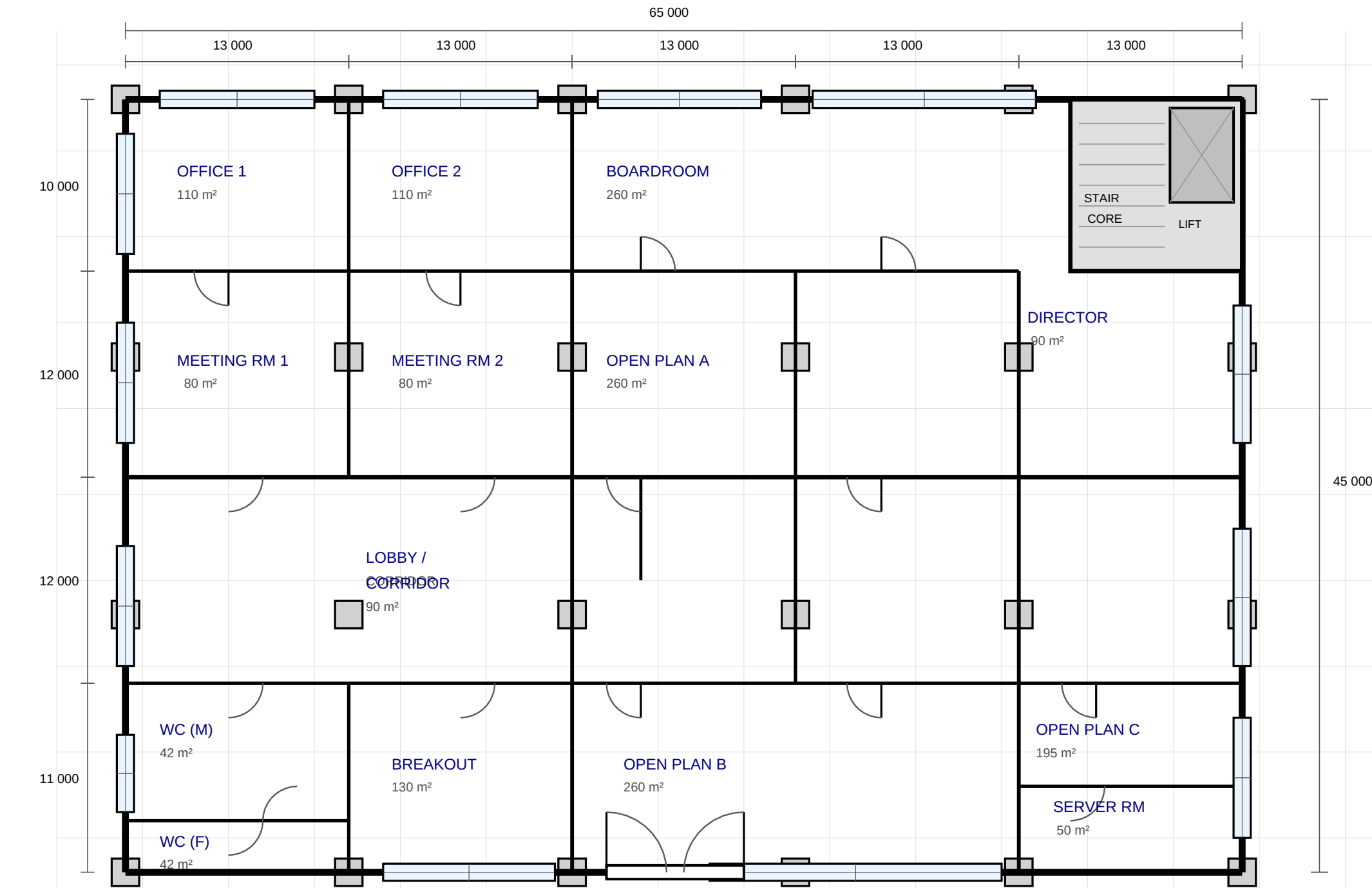
GROUND FLOOR PLAN · BLOCK A
