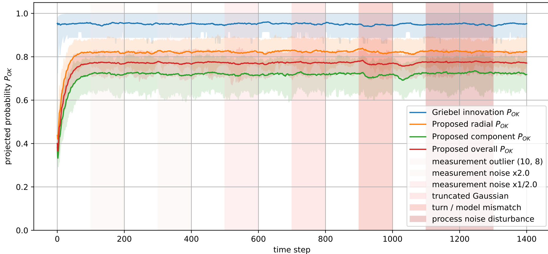
Monte Carlo mean projected probabilities, N=100
