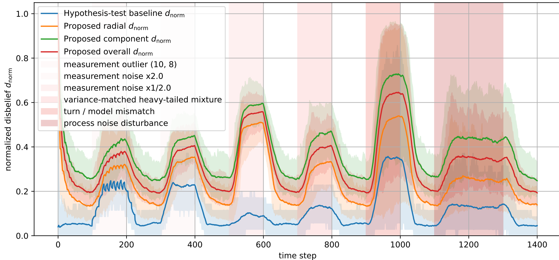
Monte Carlo mean normalized disbelief, N=100
