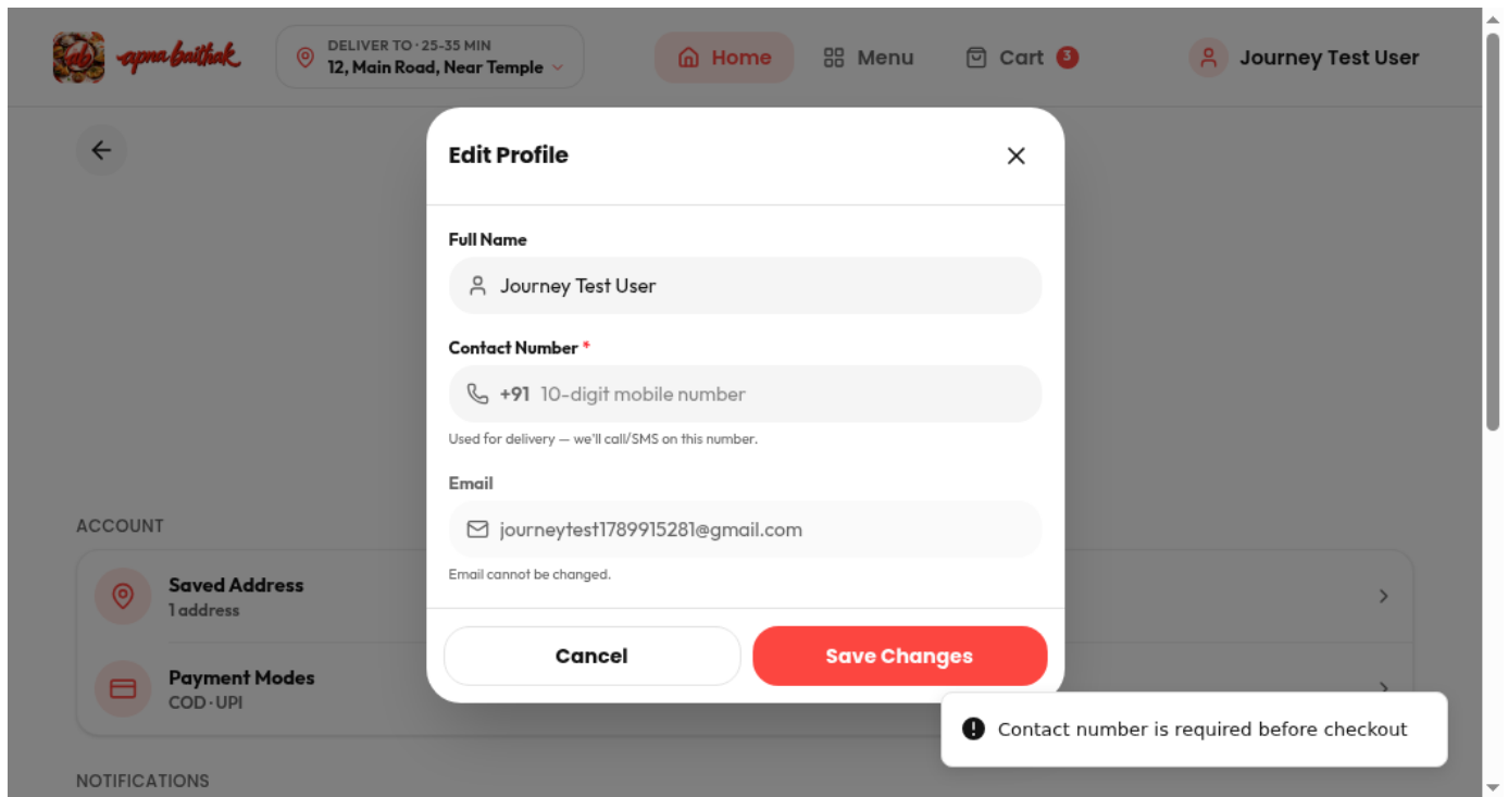
Screenshot: journey-25-checkout-payment-options.png
