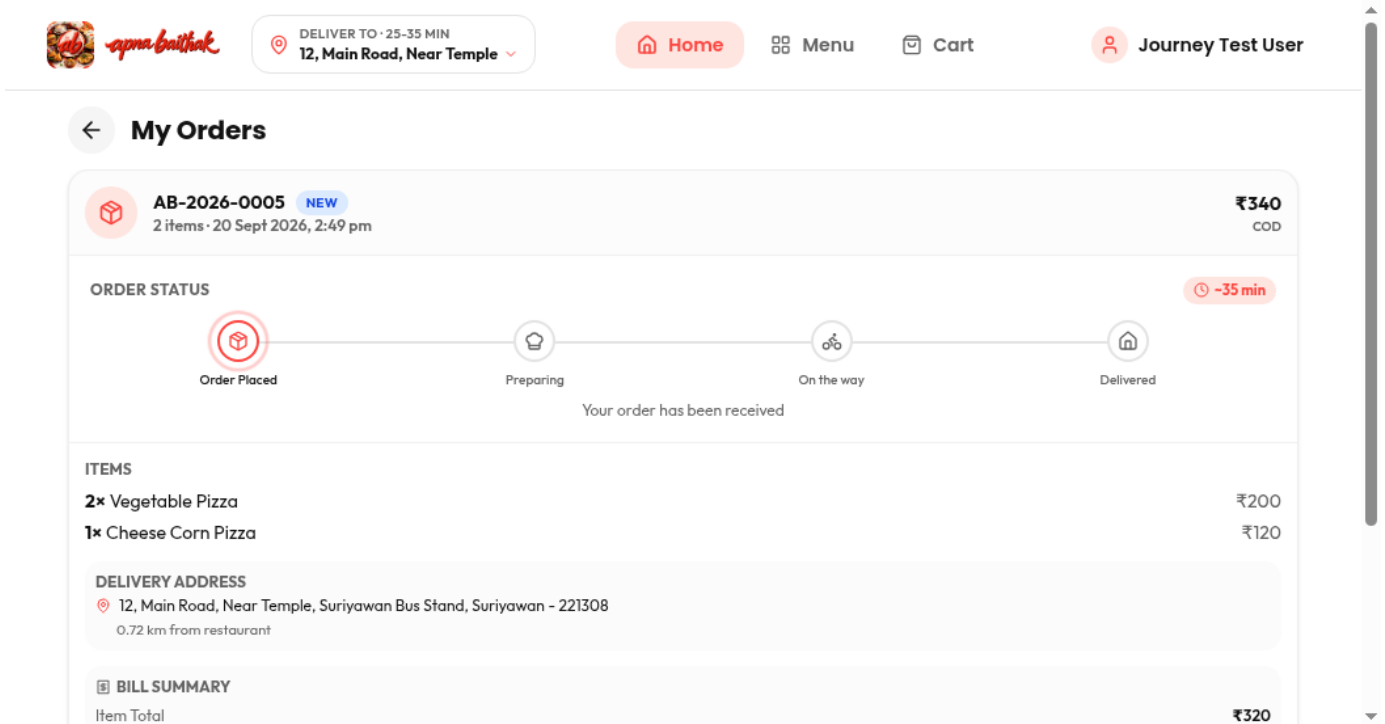
Screenshot: journey-30-order-details.png
