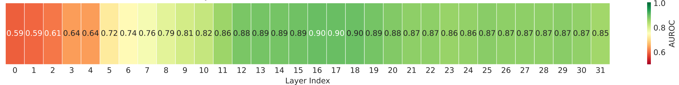
Per-Layer Hallucination Detection AUROC (LLaMA-3.1-8B)
