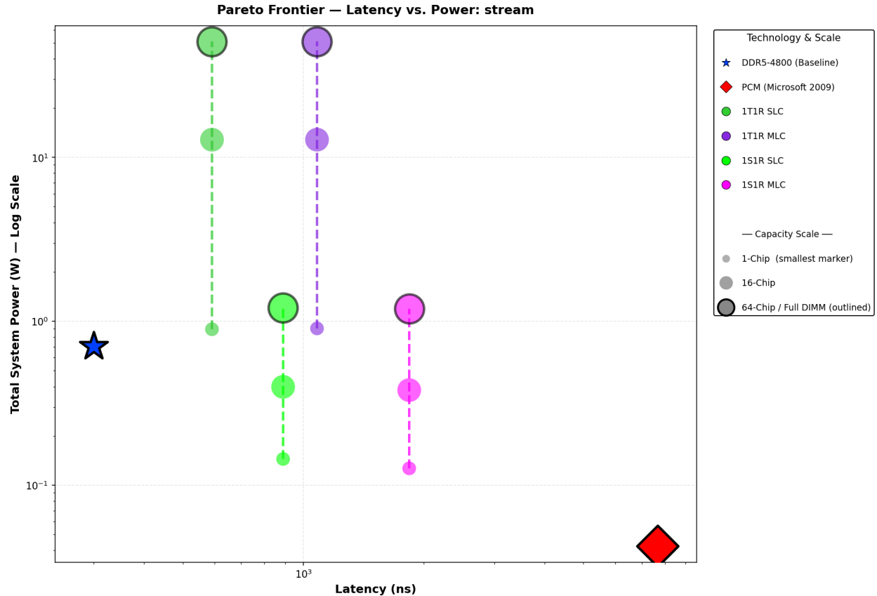
Figure 24 & 25: Pareto scaling trajectories under continuous memory-streaming workloads (LBM SPEC2017 and STREAM).
