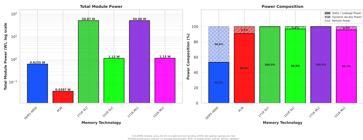
Figure 7: System Power Breakdown (Static / Dynamic / Refresh) under the compute-bound GCC (SPEC2017) workload.
