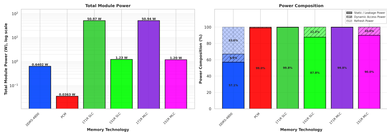
Figure 8: System Power Breakdown (Static / Dynamic / Refresh) under the highly active GPT-2 Inference (IFMAP) workload.
