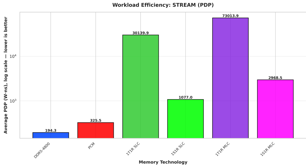
Figure 15 & 16: Power-Delay Product under heavy continuous memory-streaming workloads (LBM SPEC2017 and STREAM).
