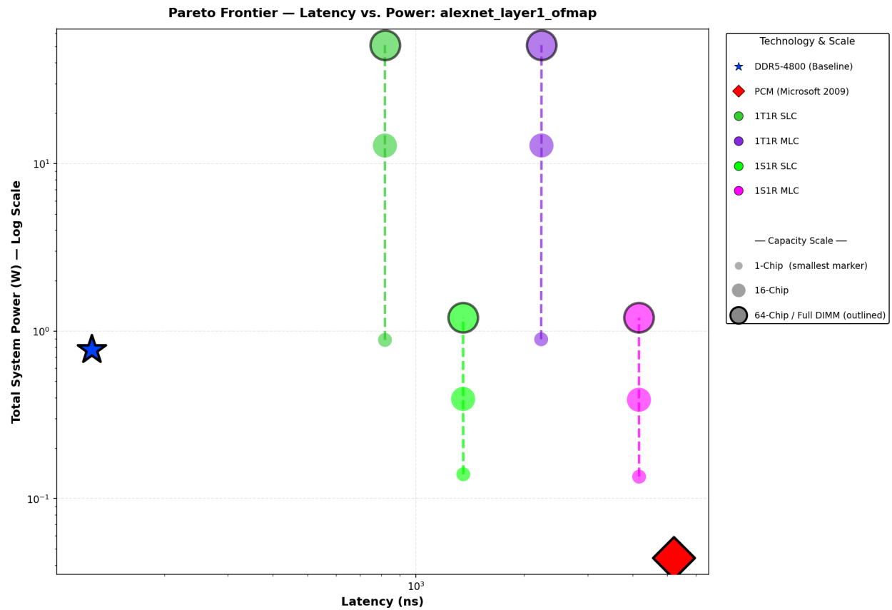
Figure 23: Pareto scaling trajectory under write-torture conditions (AlexNet OFMAP).
