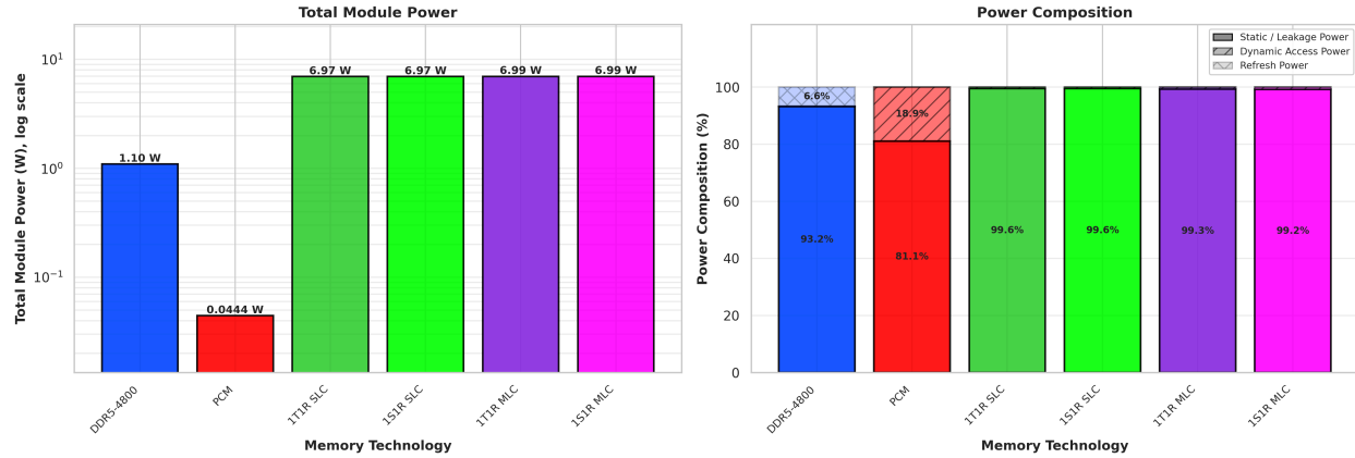
Figure 9: System Power Breakdown (Static / Dynamic / Refresh) under the continuous memory-streaming LBM (SPEC2017) workload.
