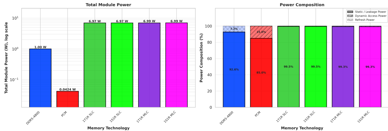
Figure 10: System Power Breakdown (Static / Dynamic / Refresh) under the STREAM benchmark.
