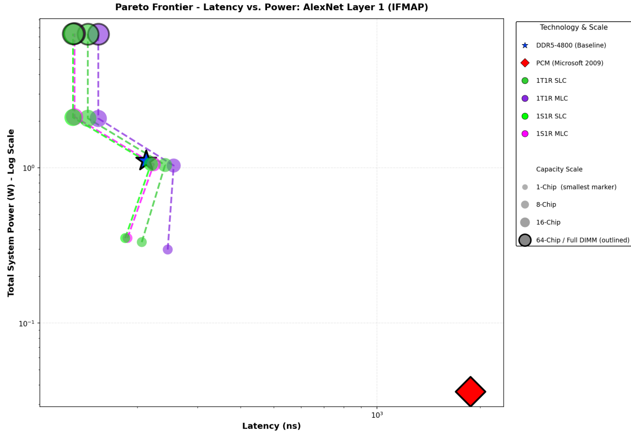
Figure 21 & 22: Pareto scaling trajectories under highly parallel AI inference workloads (GPT-2 IFMAP and AlexNet IFMAP).
