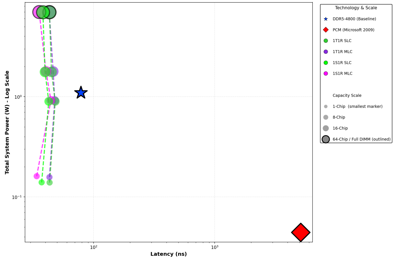
Pareto Frontier - Latency vs. Power: LBM (SPEC2017)
