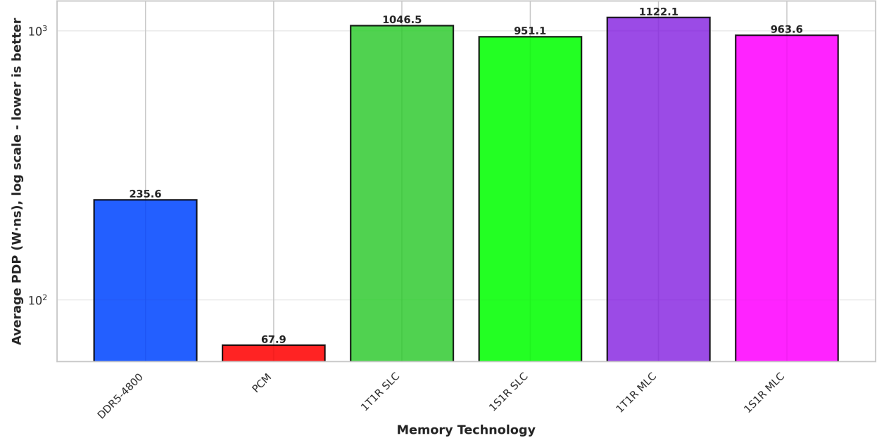
Workload Efficiency: AlexNet Layer 1 (IFMAP) (PDP)
