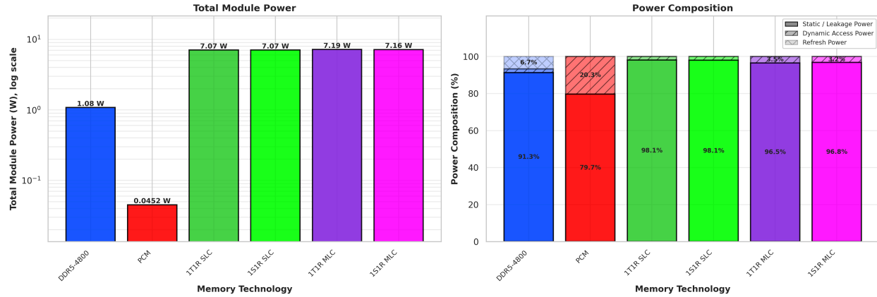
Figure 11 & 12: System Power Breakdown (Static / Dynamic / Refresh) under AlexNet Layer 1 IFMAP (Read-Heavy) and OFMAP (Write-Heavy) workloads.
