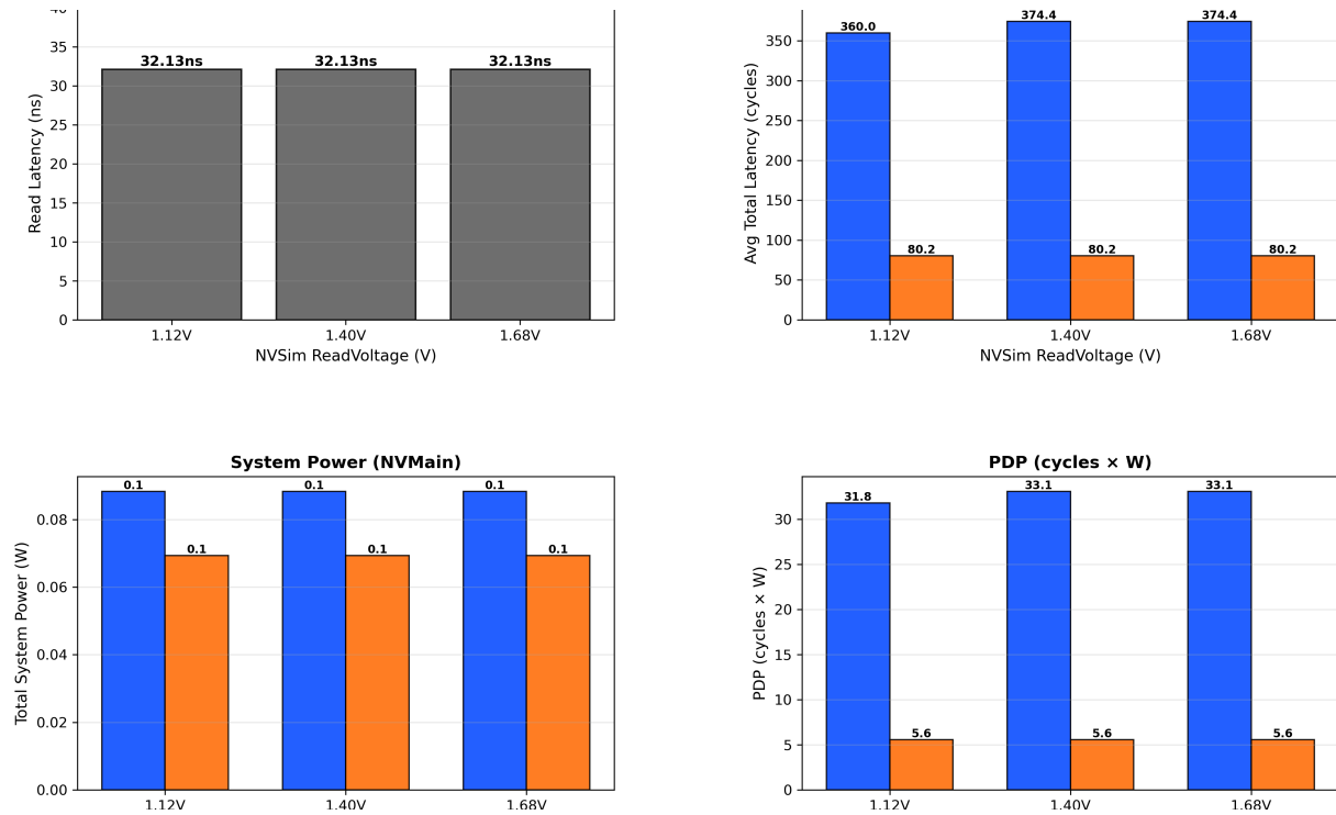
Figure 19: ReadVoltage Sensitivity Analysis - 1T1R SLC Full DIMM (LBM and GCC, +/-20% sweep), a 2 x 2 grid. Top left: NVSim circuit read latency, invariant at 32.13 ns across all three voltages. Top right: system average total latency. Bottom left: system power. Bottom right: Power-Delay Product, whose largest movement across the full sweep is 3.8% (LBM, 31.80 against 33.07 cycles x W at the 1.40 V design point), so efficiency conclusions are robust to process variation in the ReadVoltage operating point.
