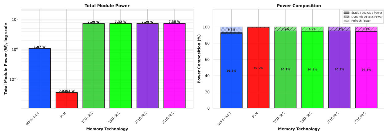
Figure 8: System Power Breakdown (Static / Dynamic / Refresh) under the highly active GPT-2 Inference (IFMAP) workload.
