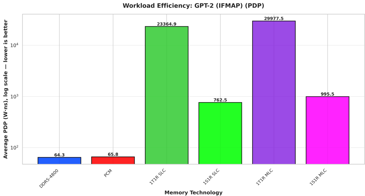
Figure 13 & 14: Power-Delay Product under single-threaded compute (GCC SPEC2017) and massively parallel AI inference (GPT-2 IFMAP) workloads.
