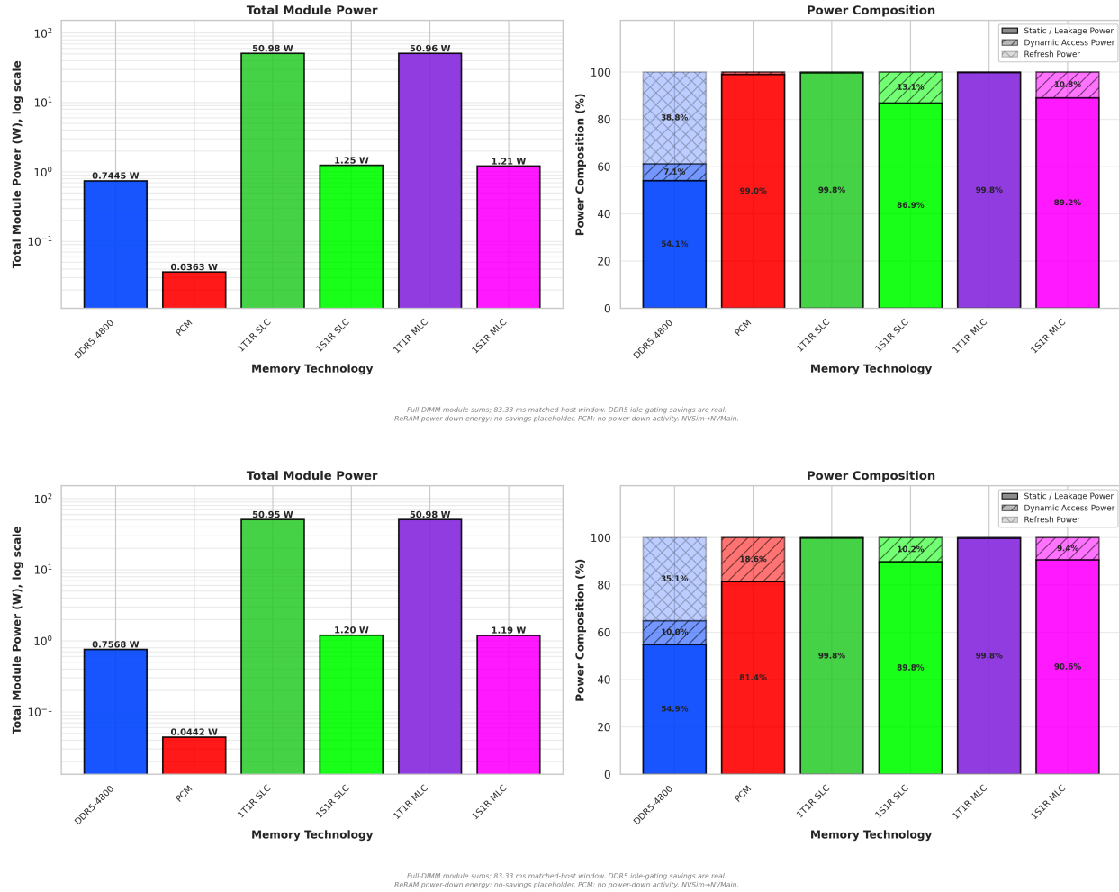
Figure 11 & 12: System Power Breakdown (Static / Dynamic / Refresh) under AlexNet Layer 1 IFMAP (Read-Heavy) and OFMAP (Write-Heavy) workloads.
