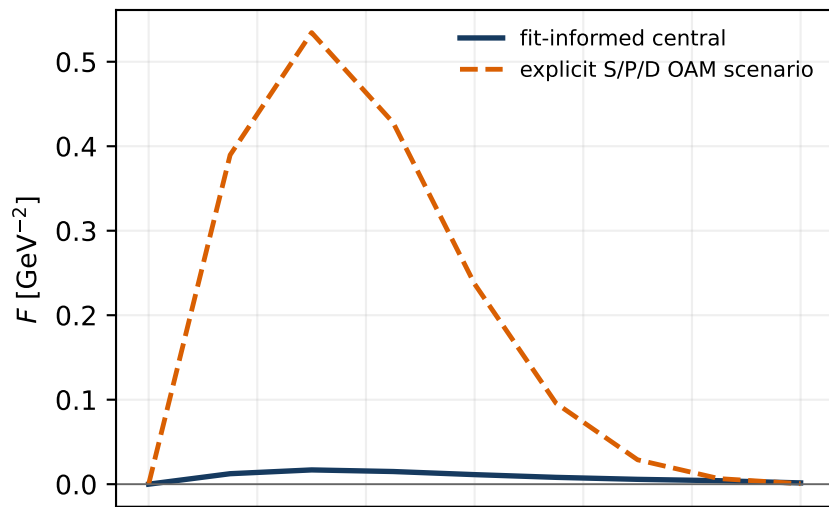
AV18 parent: f1Tperp at x_N = 0.1 , Q = 5 GeV (future link)
