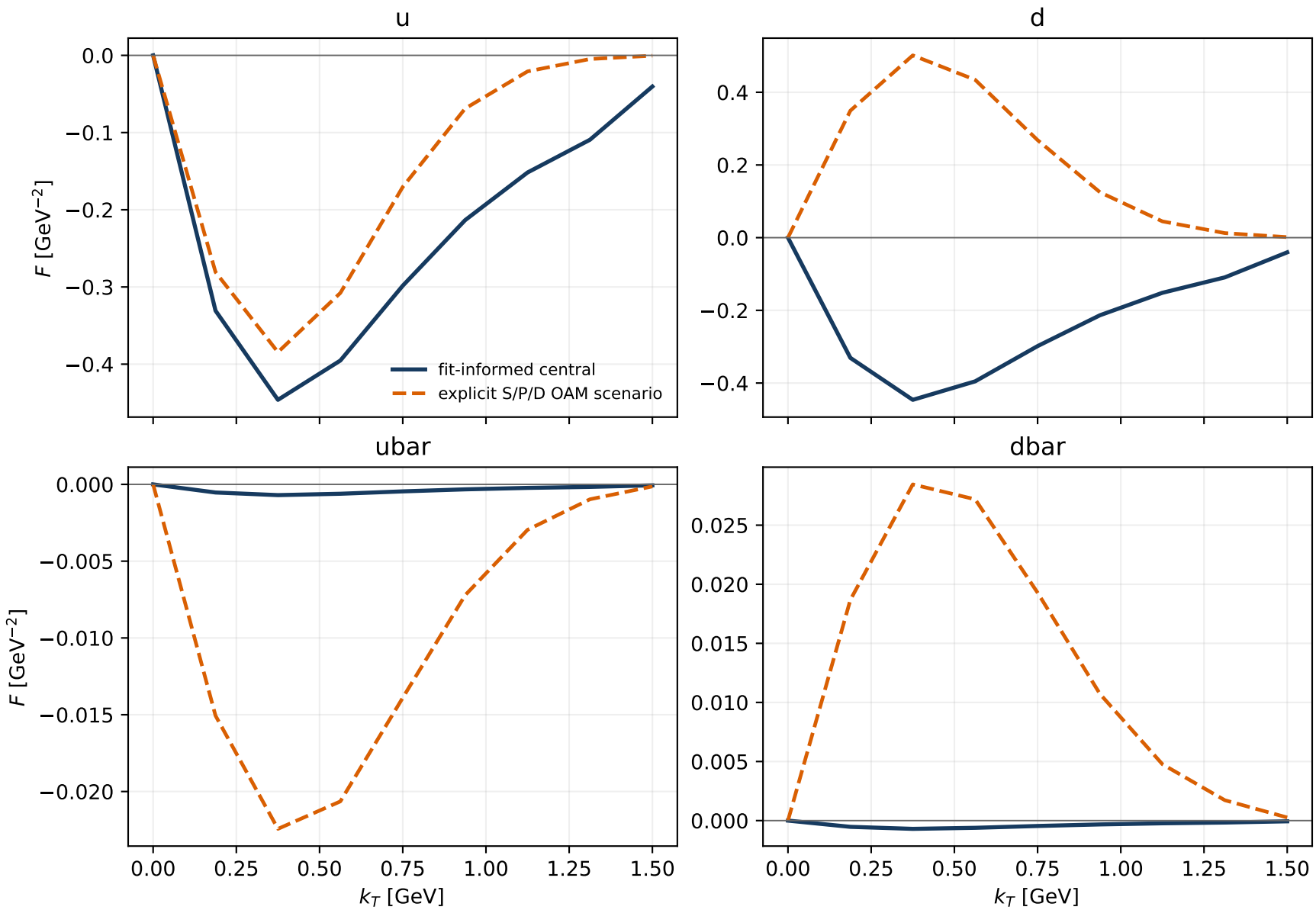
AV18 parent: h1perp at x_N = 0.1 , Q = 5 GeV (future link)
