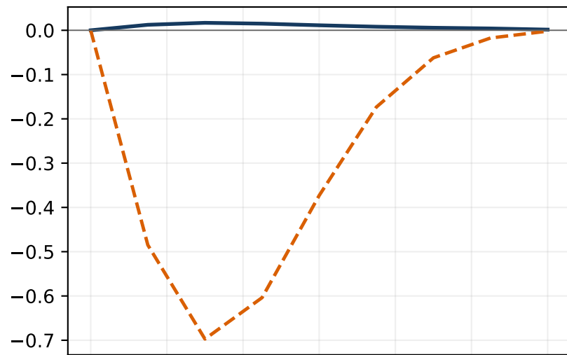
AV18 parent: f1Tperp at x_N = 0.1 , Q = 5 GeV (future link)
