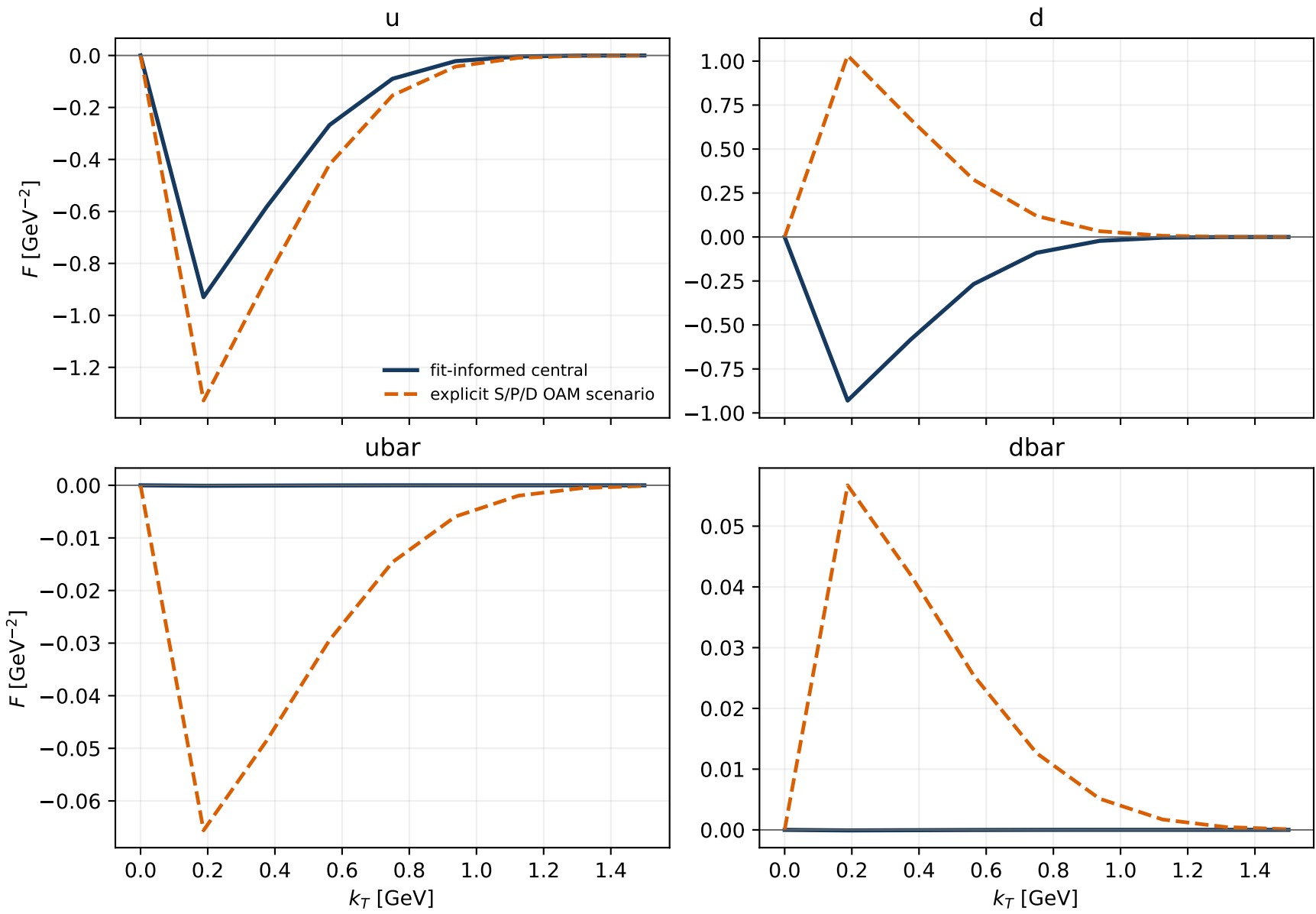
AV18 parent: h1Lperp at x_N = 0.1 , Q = 5 GeV (future link)
