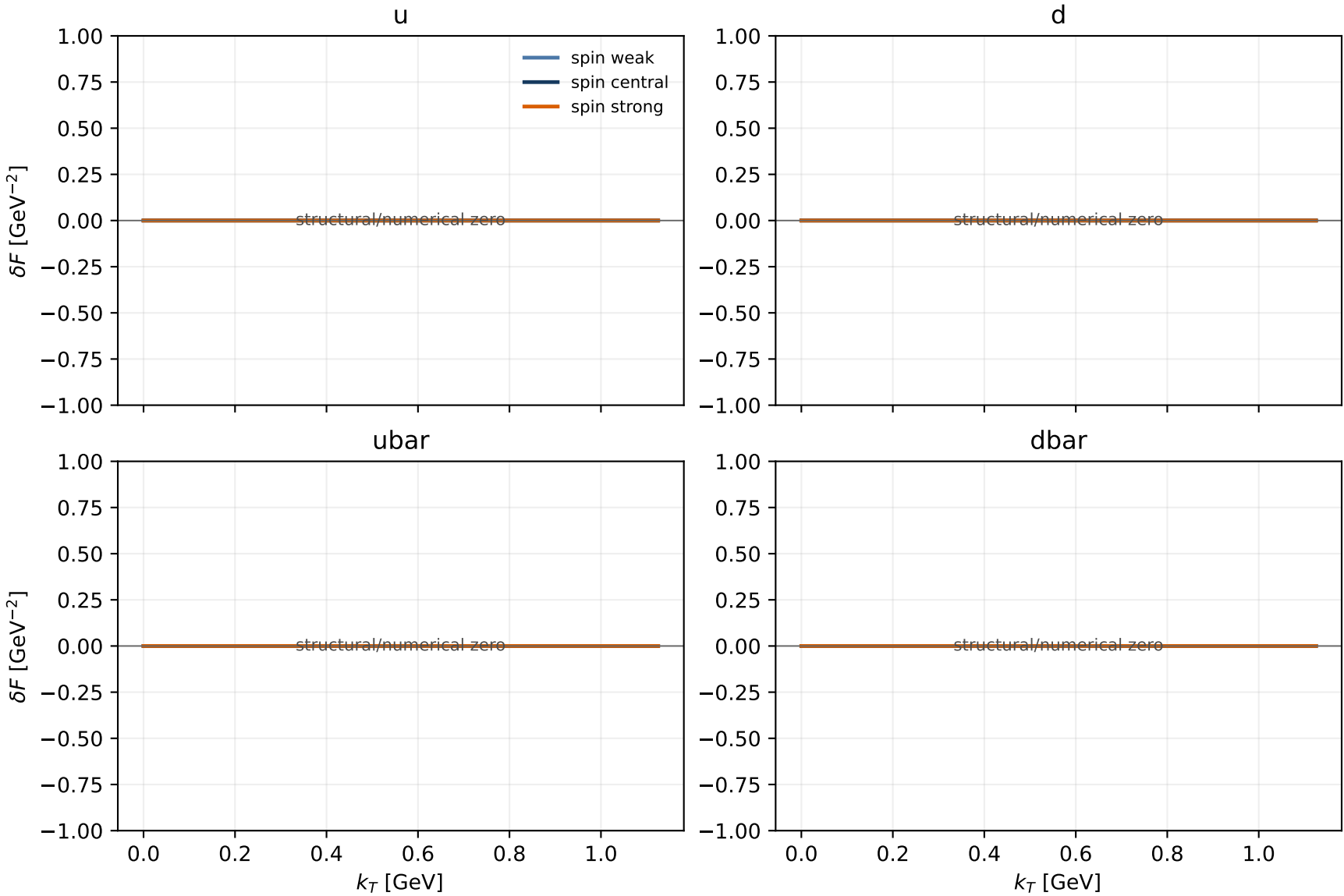
AV18 coherent quark shadowing: g1LT, x_N = 0.01 , Q = 5 GeV display restricted to the numerically resolved k_T \leq 1.2 GeV domain
