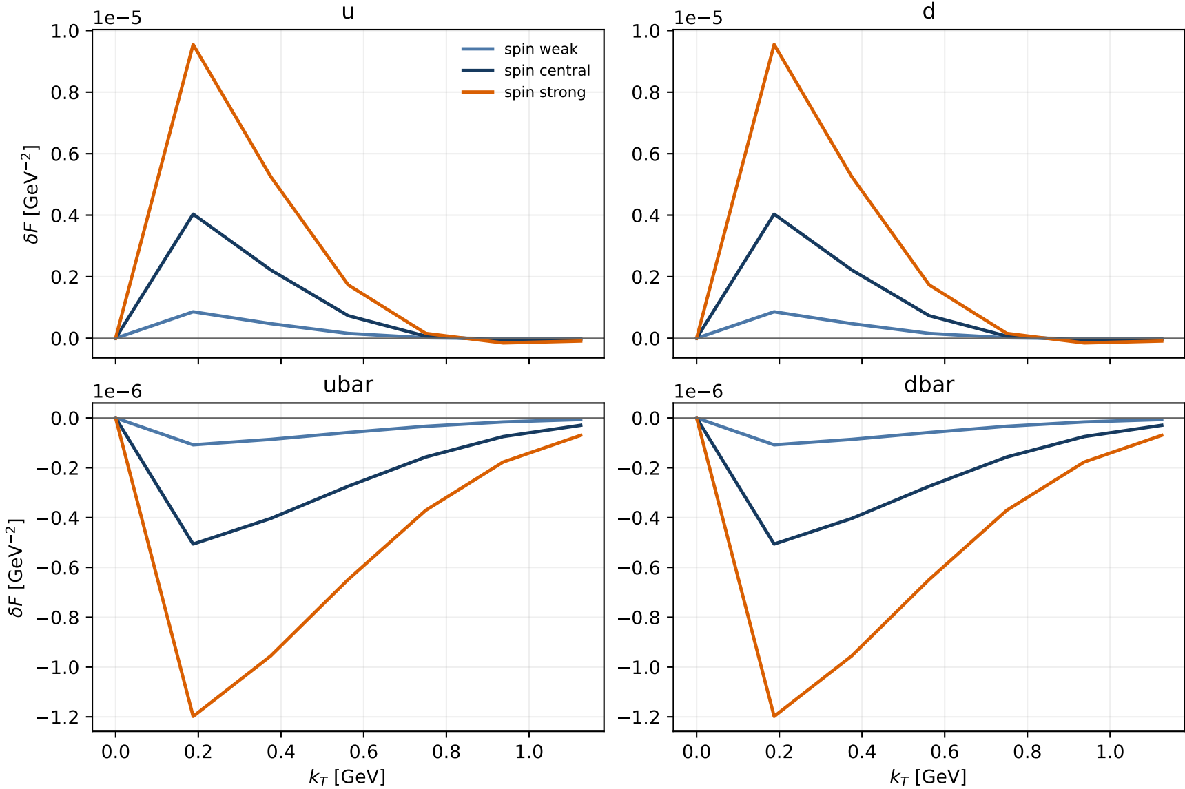
AV18 coherent quark shadowing: g1T , x_N = 0.01 , Q = 5 GeV display restricted to the numerically resolved k_T \lesssim 1.2 GeV domain
