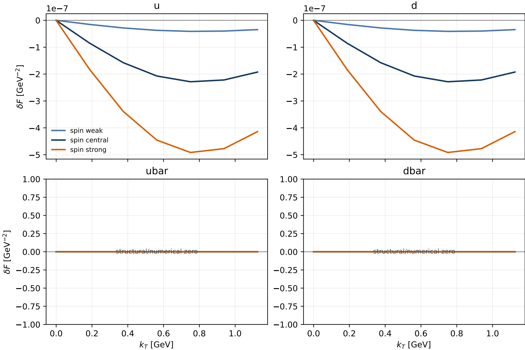
AV18 coherent quark shadowing: h1LT, x_N = 0.01 , Q = 5 GeV display restricted to the numerically resolved k_T \leq 1.2 GeV domain
