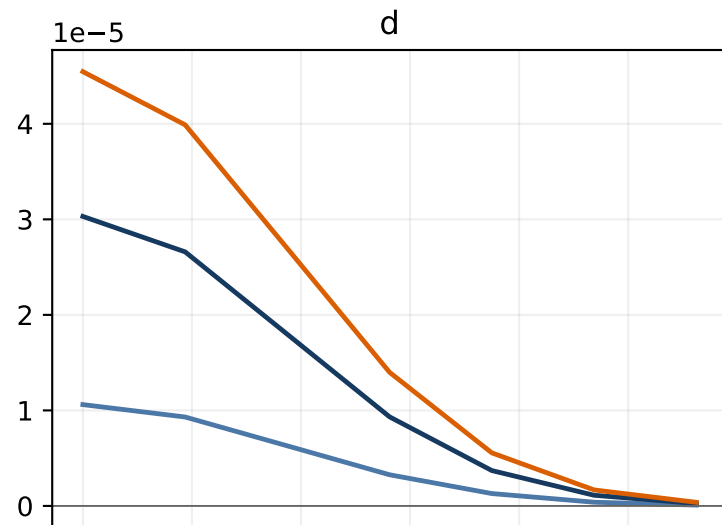
AV18 coherent quark shadowing: f1LL, x_N = 0.01 , Q = 5 GeV display restricted to the numerically resolved k_T \leq 1.2 GeV domain
