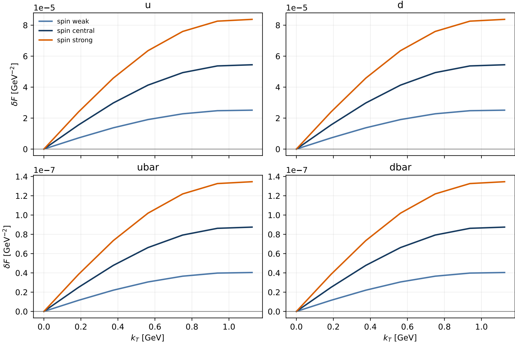
AV18 coherent quark shadowing: f1Tperp, x_N = 0.01 , Q = 5 GeV display restricted to the numerically resolved k_T \leq 1.2 GeV domain
