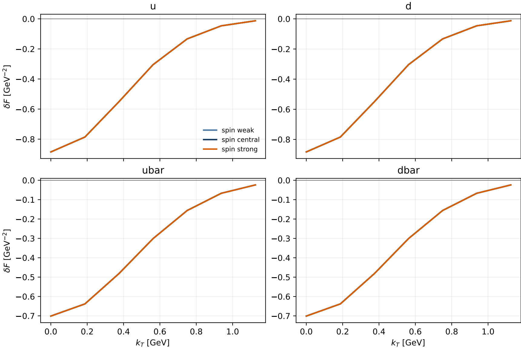
AV18 coherent quark shadowing: f1, x_N = 0.01 , Q = 5 GeV display restricted to the numerically resolved k_T \lesssim 1.2 GeV domain
