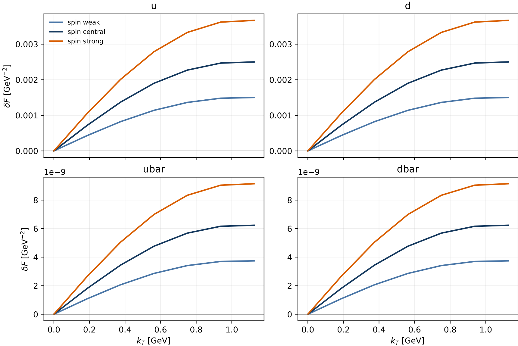
AV18 coherent quark shadowing: h1perp, x_N = 0.01 , Q = 5 GeV display restricted to the numerically resolved k_T \leq 1.2 GeV domain
