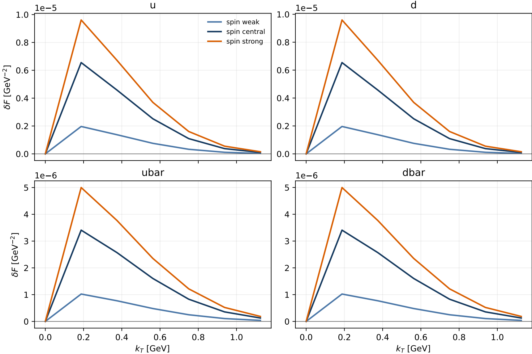
AV18 coherent quark shadowing: f1TT, x_N = 0.01 , Q = 5 GeV display restricted to the numerically resolved k_T \leq 1.2 GeV domain
