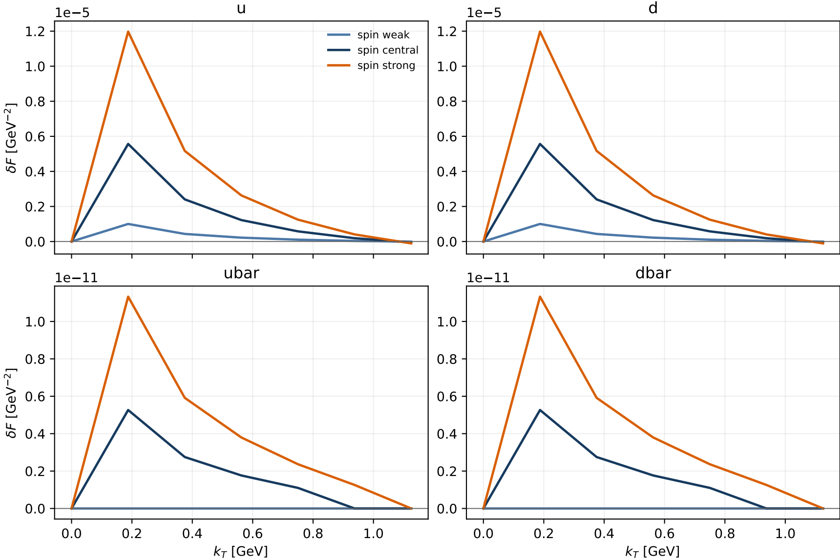
AV18 coherent quark shadowing: h1LTperp, x_N = 0.01 , Q = 5 GeV display restricted to the numerically resolved k_T \leq 1.2 GeV domain
