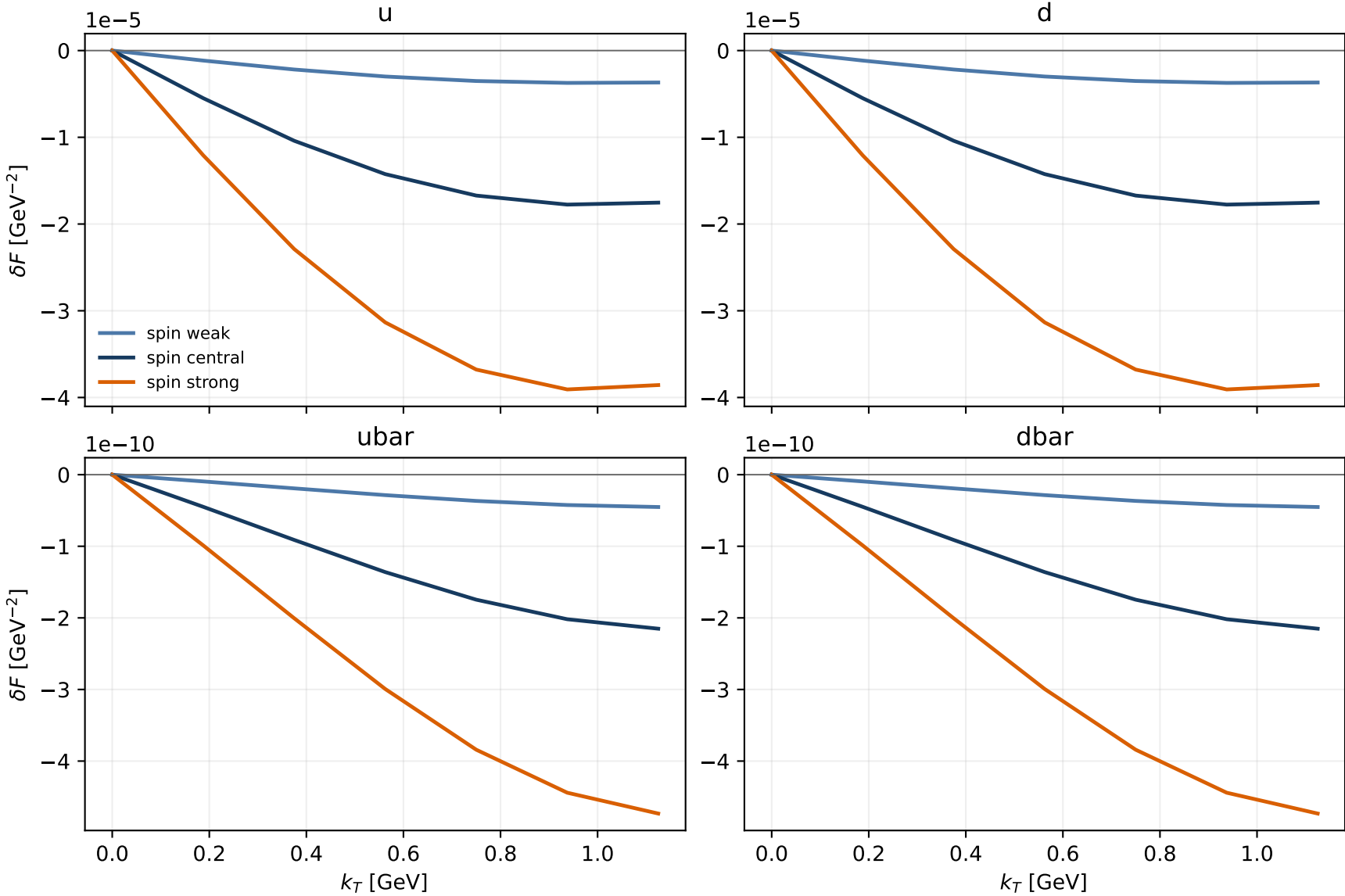
AV18 coherent quark shadowing: h1LLperp, x_N = 0.01 , Q = 5 GeV display restricted to the numerically resolved k_T \leq 1.2 GeV domain
