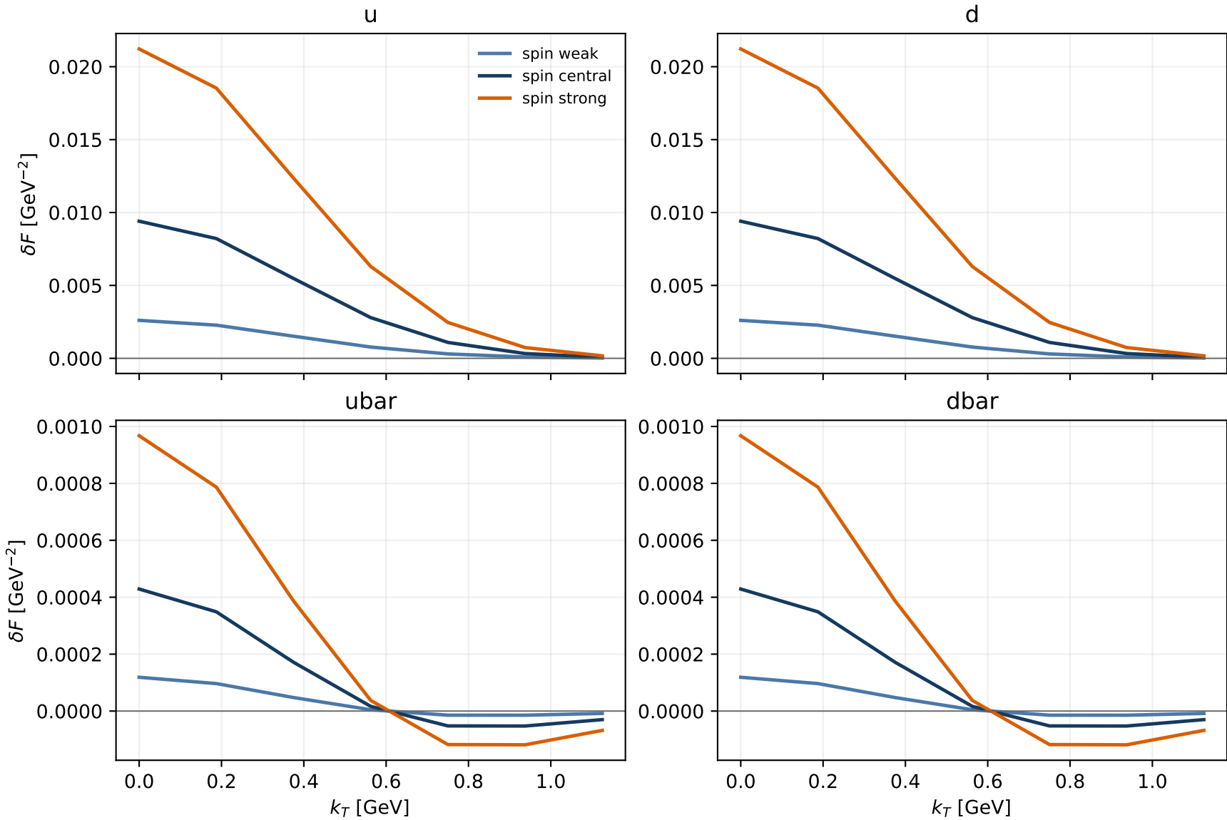
AV18 coherent quark shadowing: h1, x_N = 0.01 , Q = 5 GeV display restricted to the numerically resolved k_T \lesssim 1.2 GeV domain
