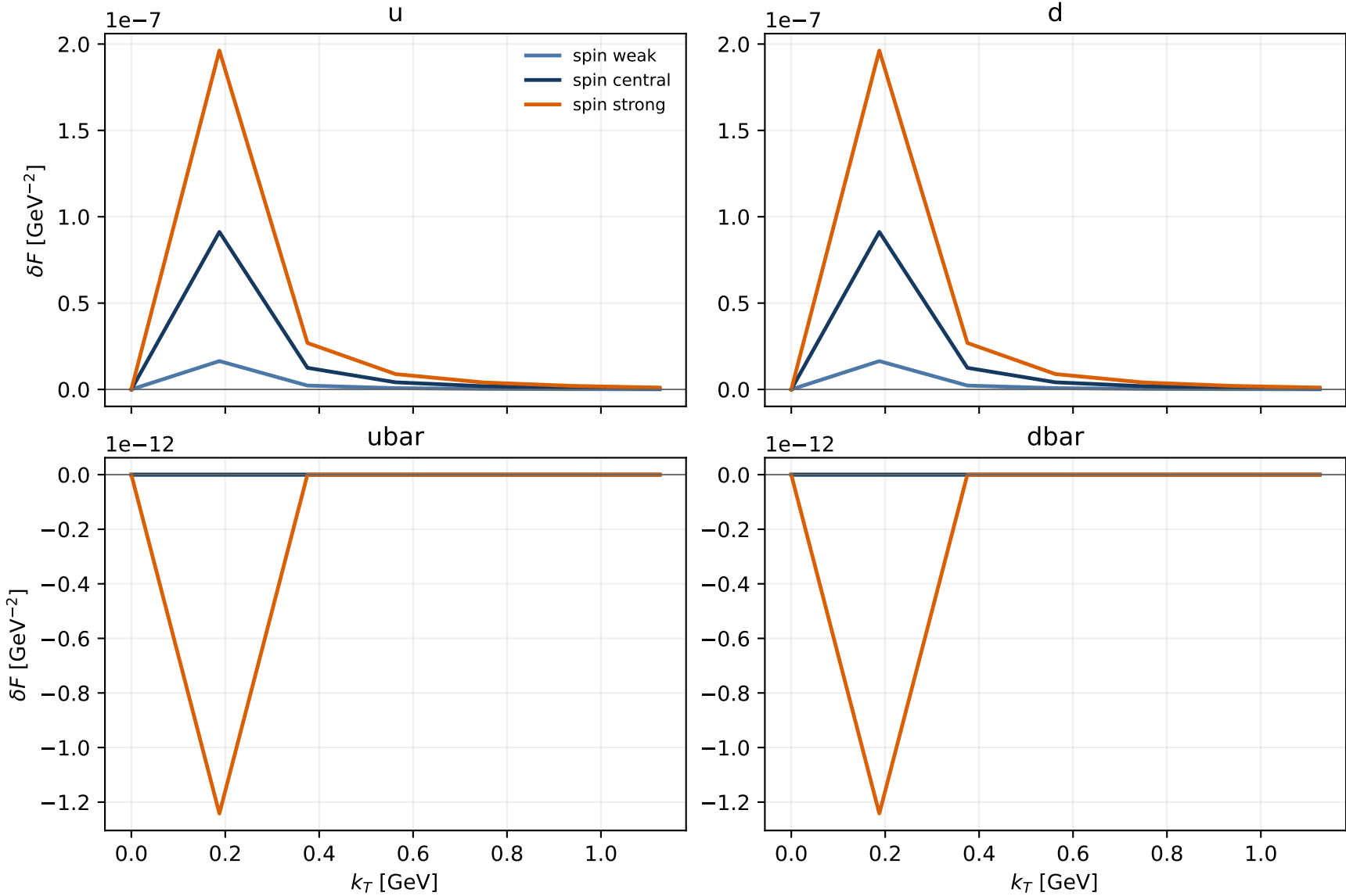
AV18 coherent quark shadowing: h1TTperp, x_N = 0.01 , Q = 5 GeV display restricted to the numerically resolved k_T \leq 1.2 GeV domain
