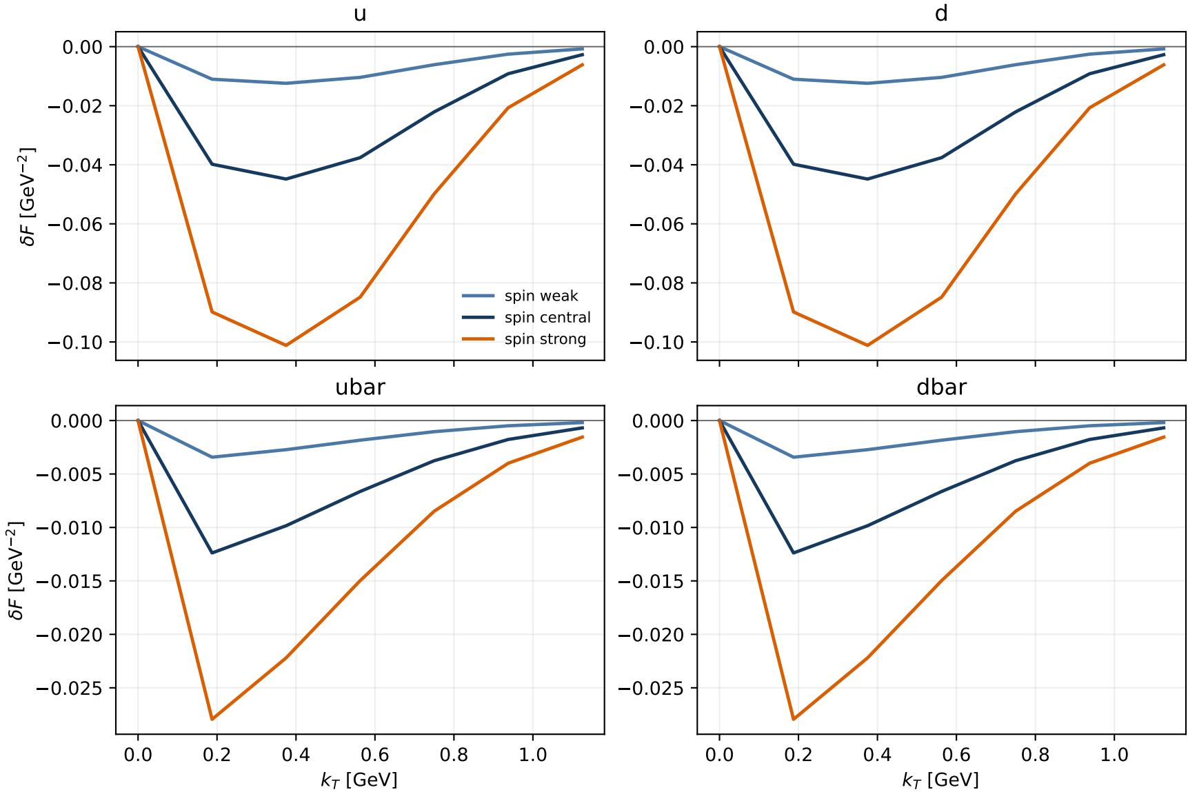
AV18 coherent quark shadowing: h1Tperp, x_N = 0.01 , Q = 5 GeV display restricted to the numerically resolved k_T \lesssim 1.2 GeV domain
