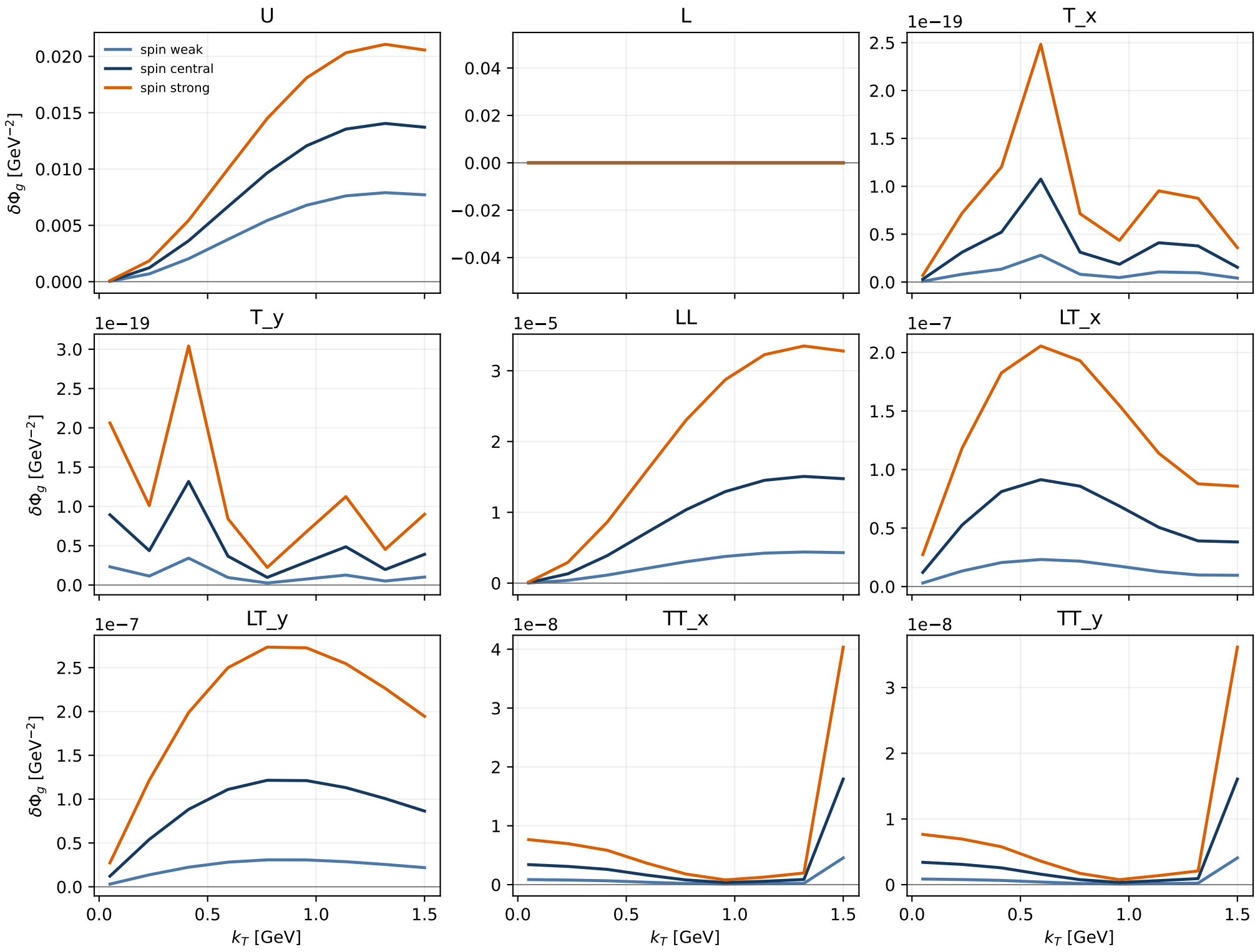
AV18 coherent shadowing: linear-polarization norm, x_N = 0.01 , Q = 5 GeV
