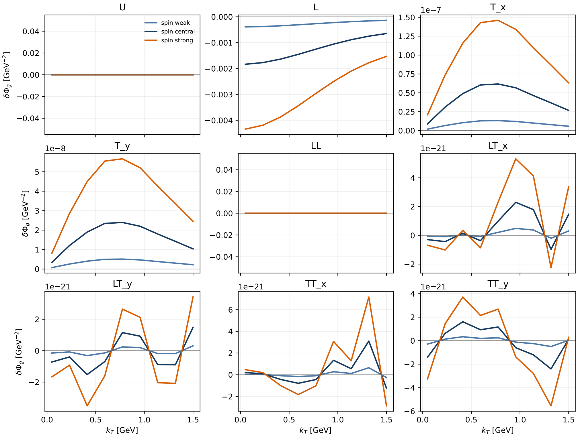
AV18 coherent shadowing: circular gluon polarization, x_N = 0.01 , Q = 5 GeV
