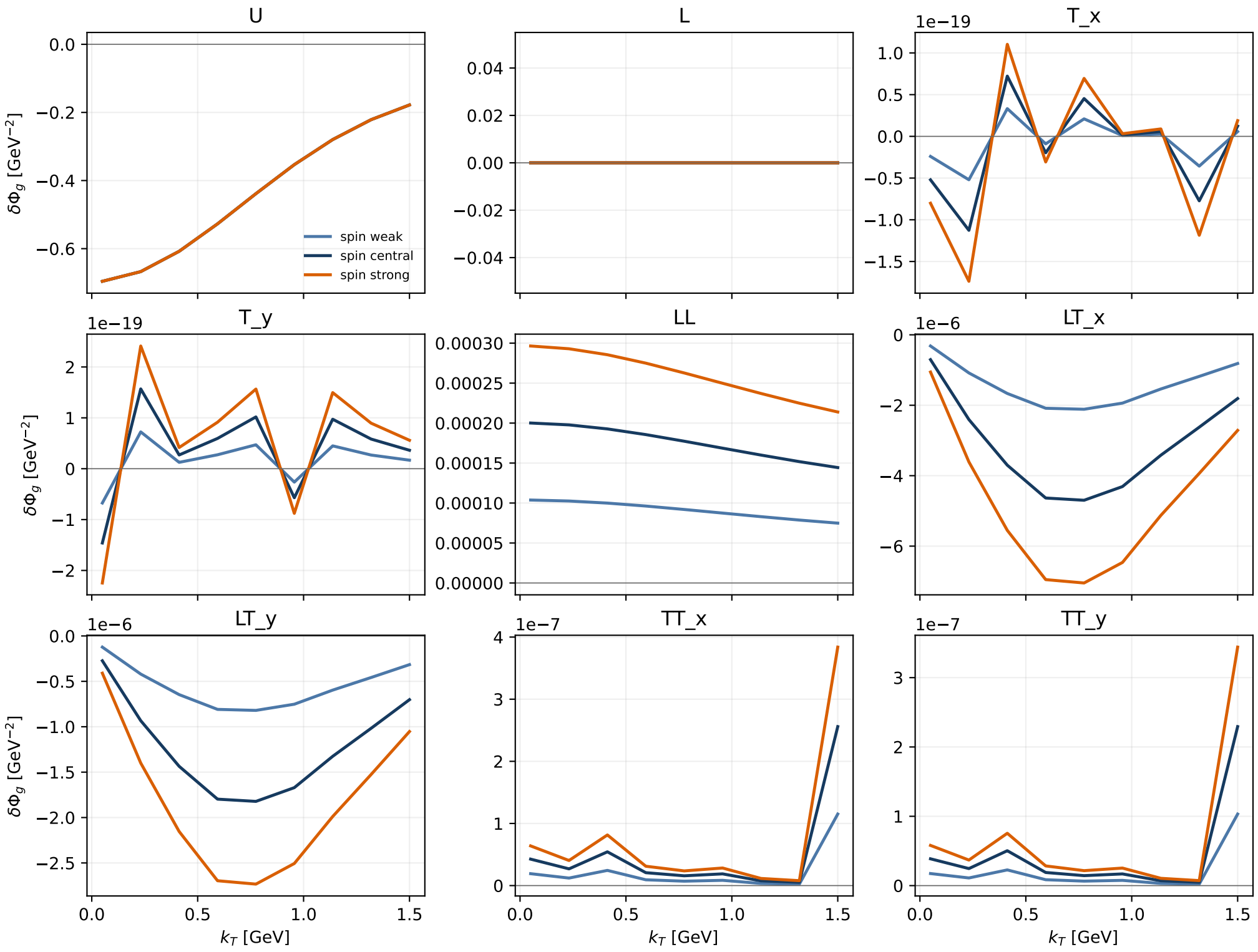
AV18 coherent shadowing: gluon trace, x_N = 0.01 , Q = 5 GeV
