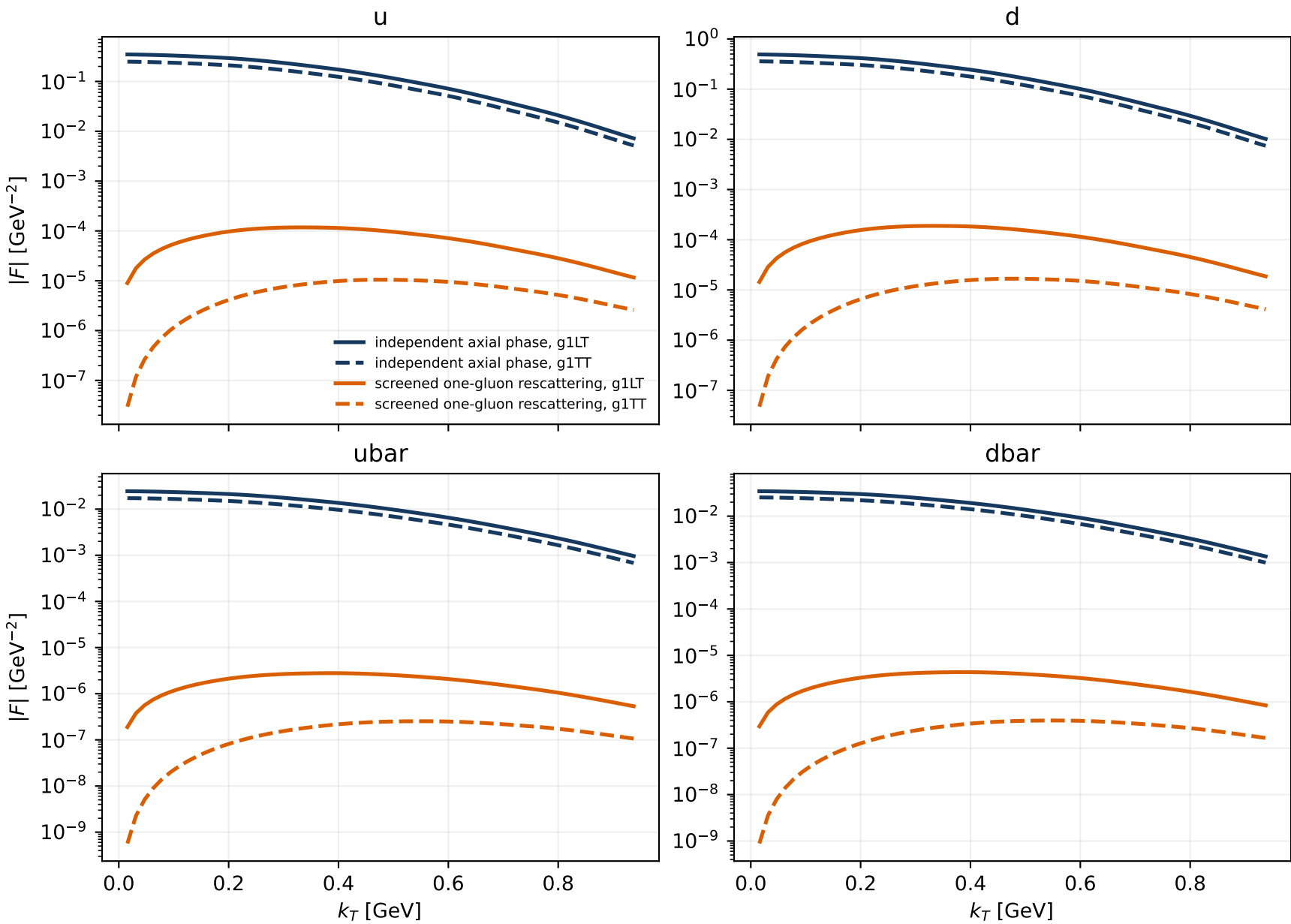
Central two-stage magnitude comparison, x_N = 0.1 , Q = 5 GeV, AV18
