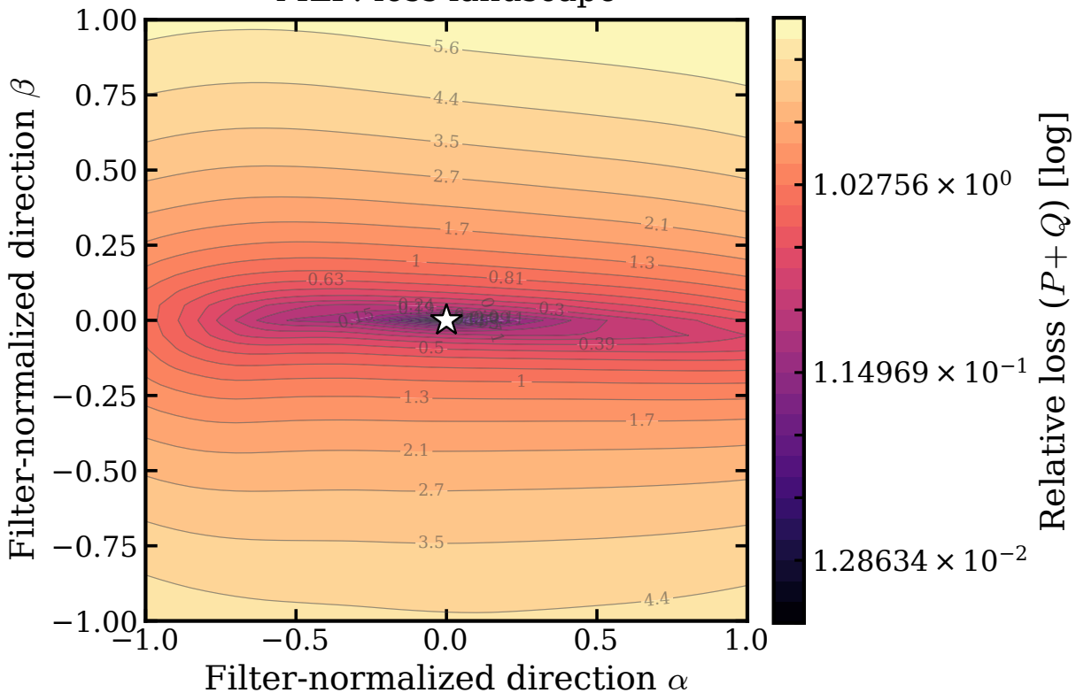
MLP: loss landscape
