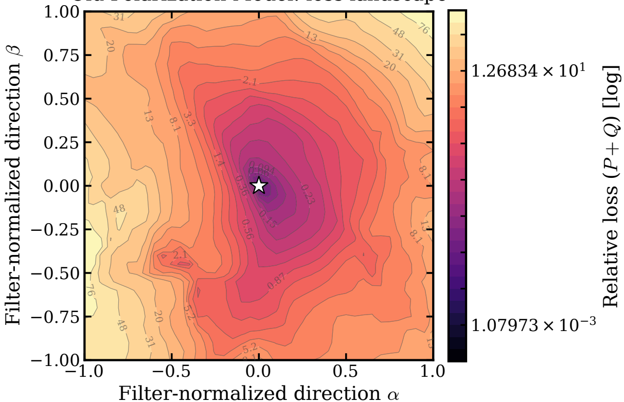
Old Polarization Model: loss landscape
