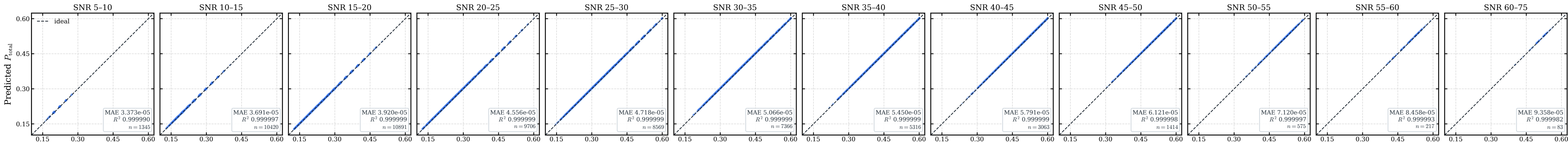
Transformer: predicted vs true by SNR
