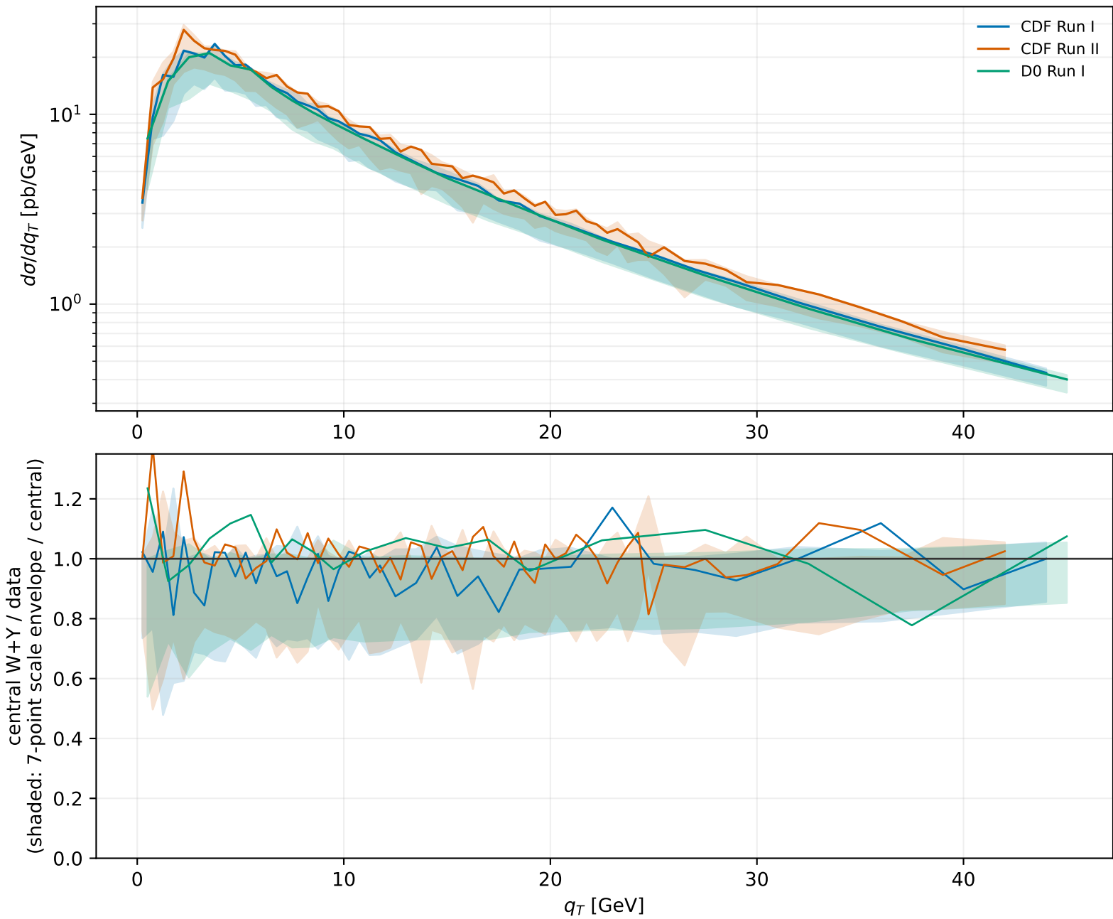
Unprimed N 3 LL+NNLO Tevatron W + Y: scale envelope
