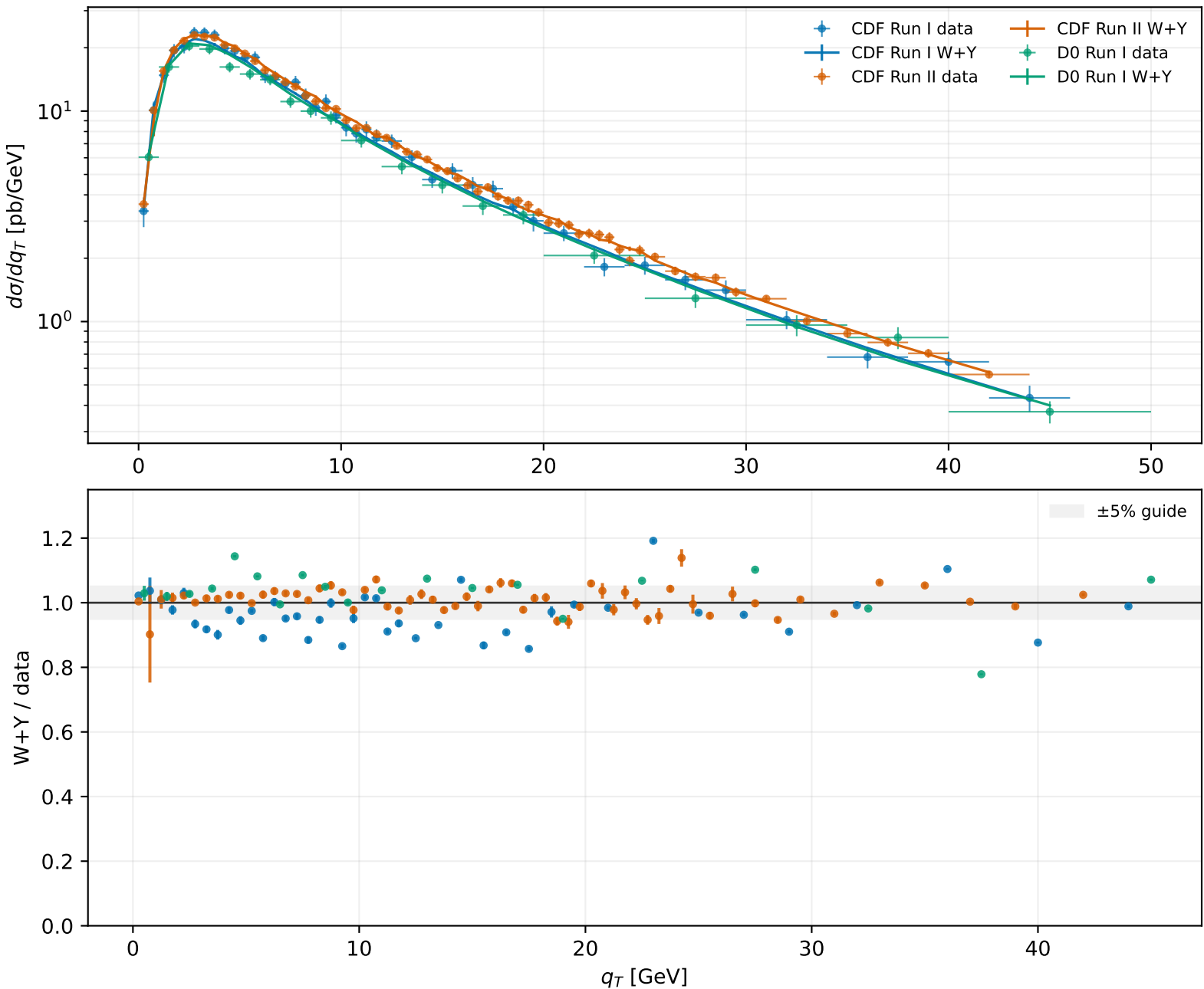
Unprimed N 3 LL+NNLO conventional W + Y Tevatron candidate
