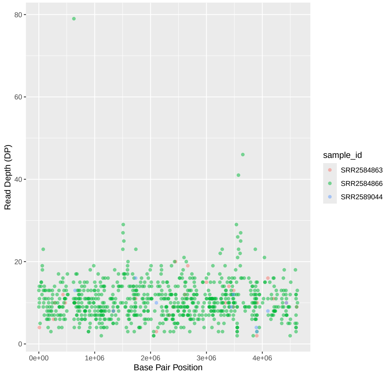
Read Depth vs. Position
