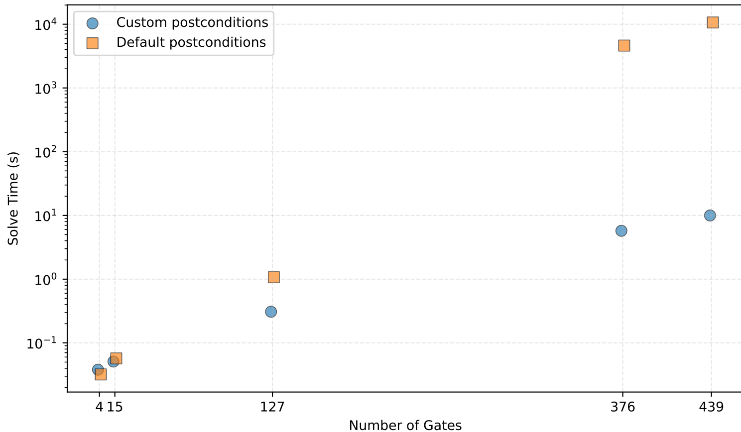
Gate Count vs Solve Time for GMW Circuits
