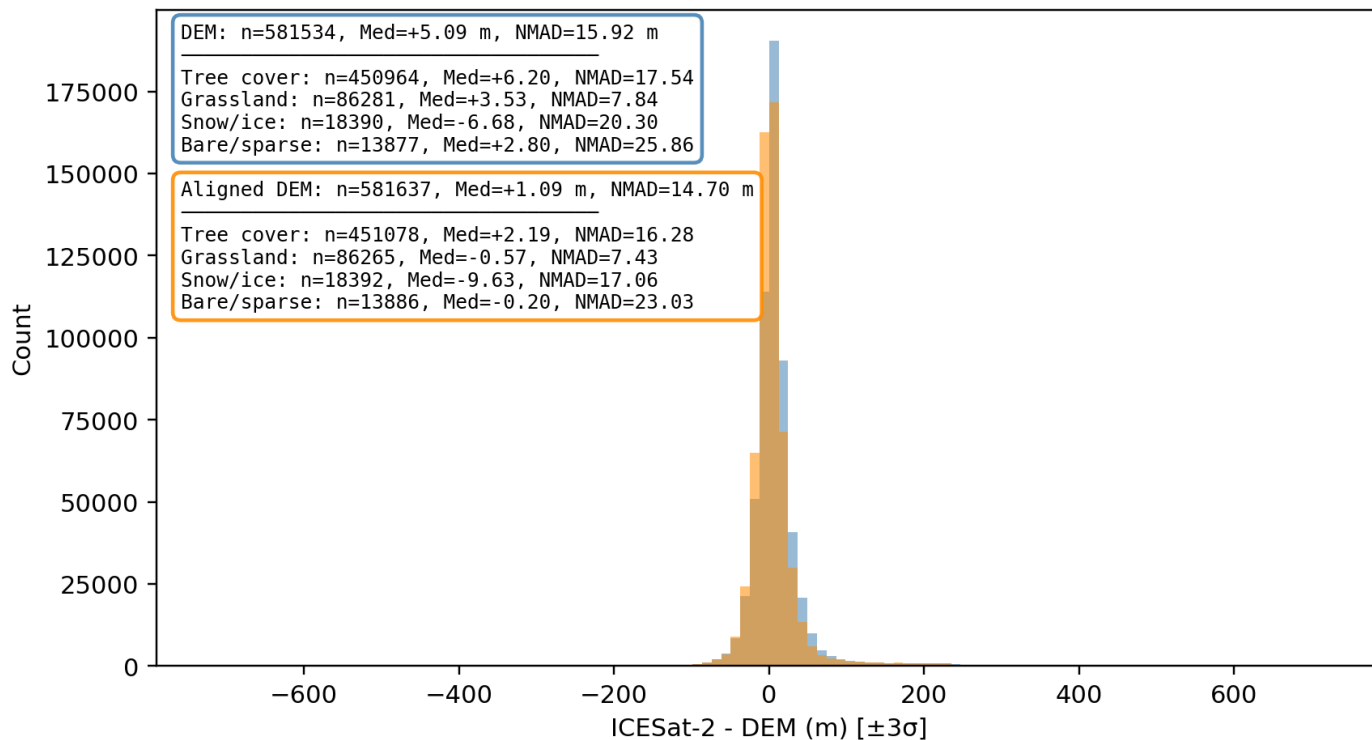
Figure 11: Pre- (steelblue) and post-alignment (orange) distributions of ICESat-2 minus DEM height differences, with per-landcover statistics in the two stacked text boxes. Box outline color matches the bar color.
