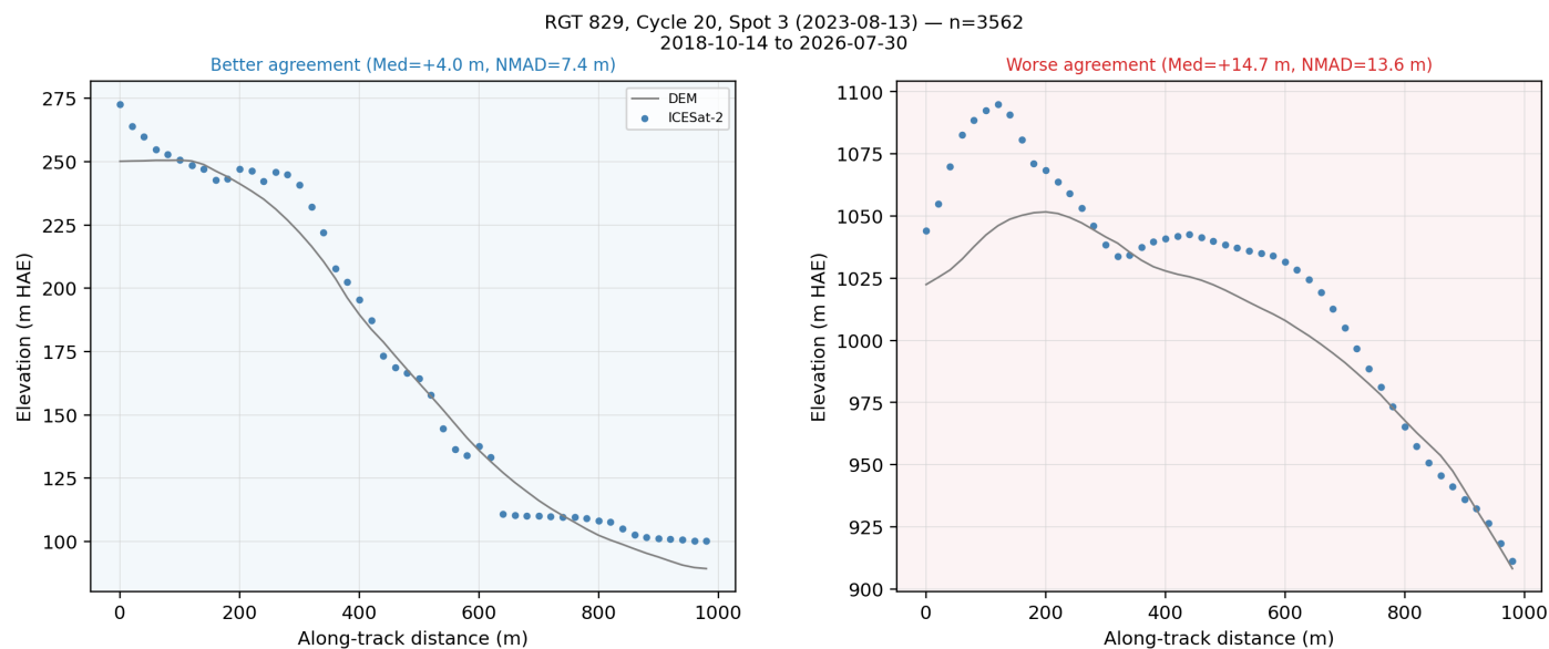
Figure 10: 1 km segments along the ICESat-2 track with better (left) and worse (right) agreement with the DEM. Segments are scored by 3 \cdot |\text{median}(\text{dh})| + \text{NMAD}(\text{dh}) , which weights the median bias three times more than the dispersion so that a segment with a large bias is not selected as 'better agreement' just because its NMAD is small.
