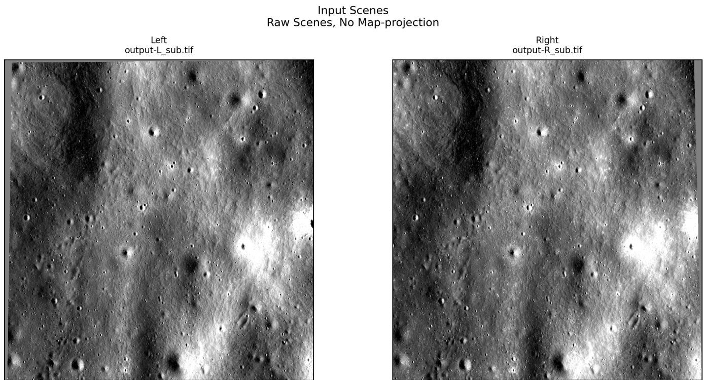
Figure 1: Left and right input scenes used for stereo processing. Non-mapprojected scenes are shown after ASP's alignment step (e.g., affineepipolar), which rotates images to create horizontal epipolar lines for correlation. Mapprojected scenes have been orthorectified with RPCs against a reference DEM to roughly align the two images prior to correlation, which reduces the disparity search range; they are displayed here in their map-projected orientation.
