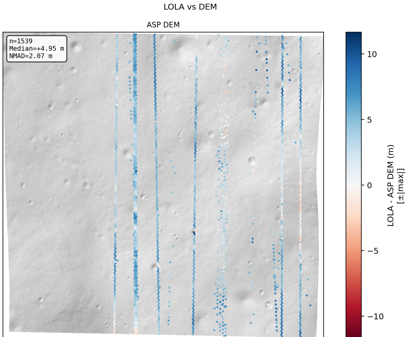
Figure 6: LOLA elevation differences vs. ASP DEM.
