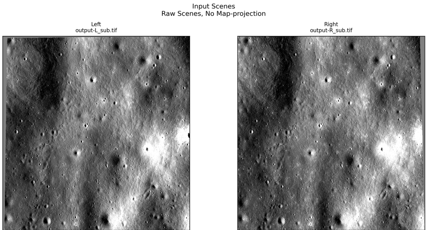
Figure 1: Left and right input scenes used for stereo processing. Non-mapprojected scenes are shown after ASP's alignment step (e.g., affineepipolar ), which rotates images to create horizontal epipolar lines for correlation. Mapprojected scenes have been orthorectified with RPCs against a reference DEM to roughly align the two images prior to correlation, which reduces the disparity search range; they are displayed here in their map-projected orientation.
