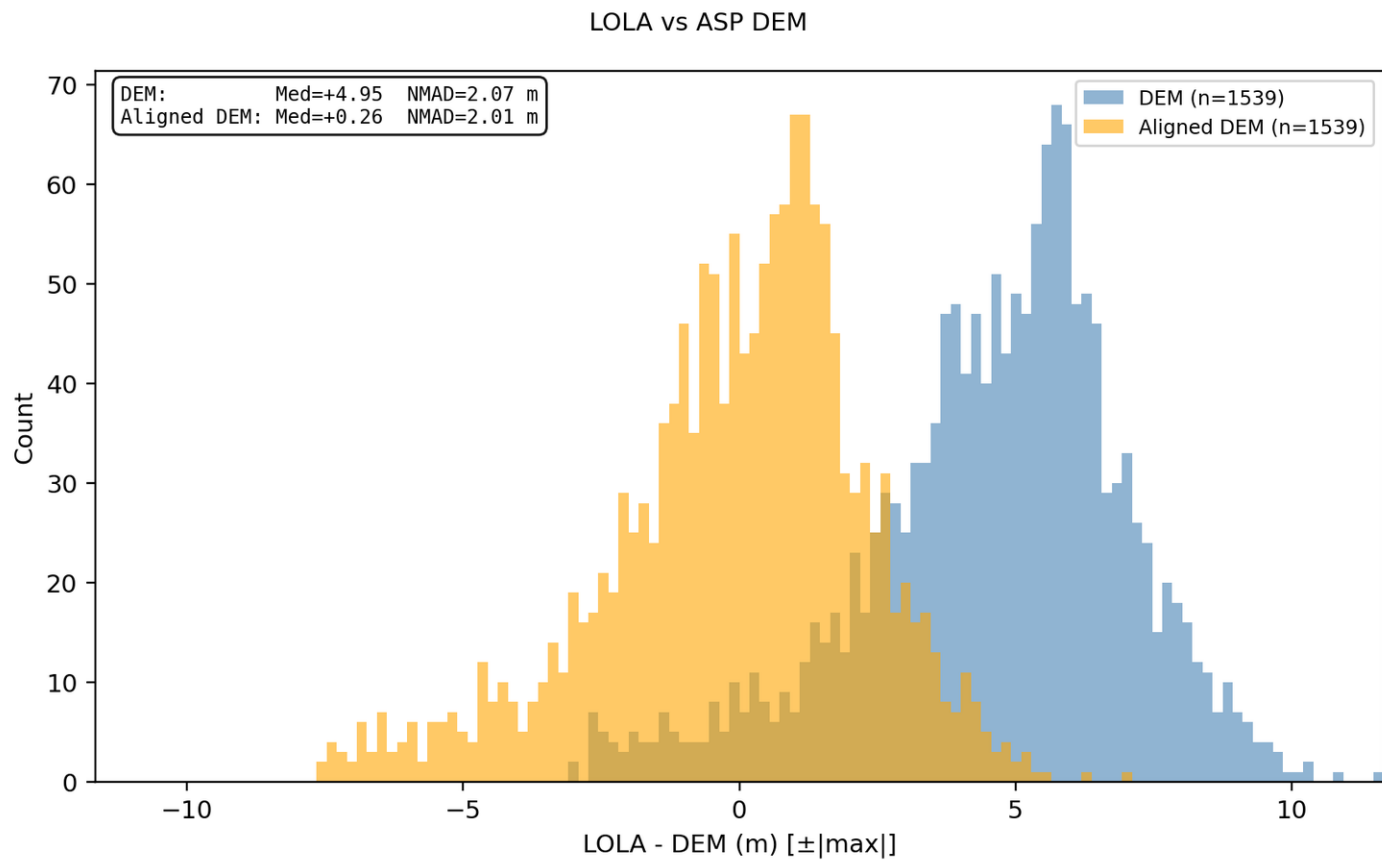
Figure 10: Pre- (steelblue) and post-alignment (orange) distributions of LOLA minus DEM height differences with shared bin edges.
