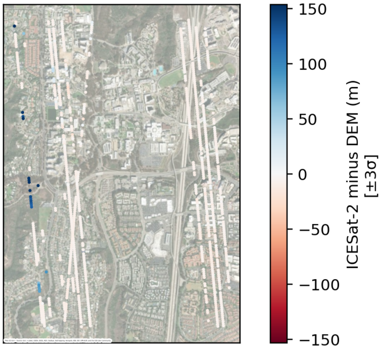
Figure 9: ICESat-2 ATL06-SR elevation differences vs. ASP DEM.
