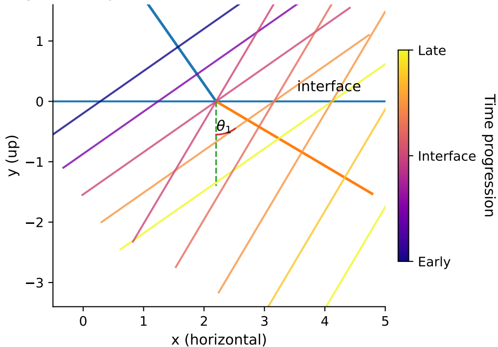
Timing continuity across an interface (Snell's law schematic)
