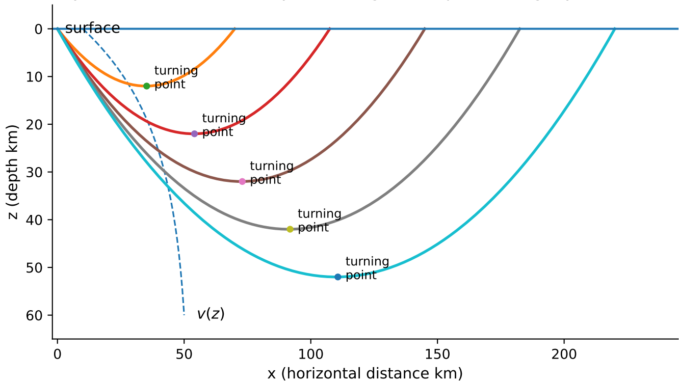
Rays in a model with velocity increasing with depth (turning rays schematic)
