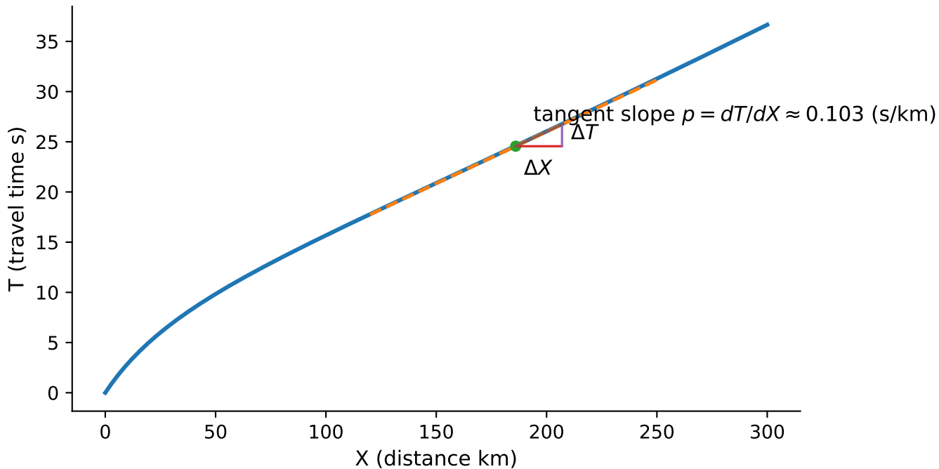
Travel-time curve and ray parameter p = dT/dX
