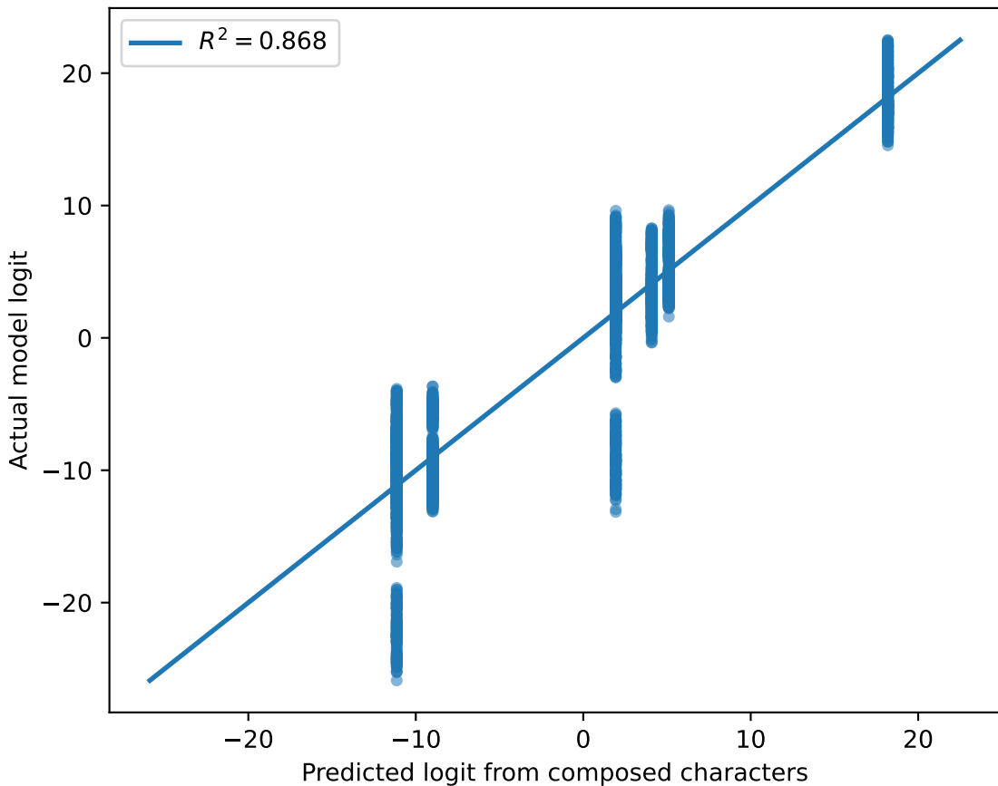
Character Logit Fit: J_{11} \cong C_2 \times C_4
