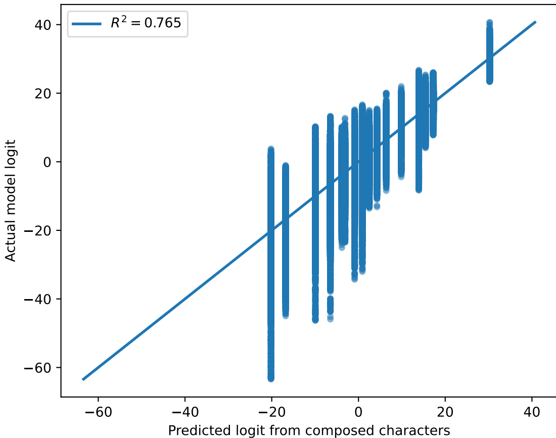
Character Logit Fit: J_3 \cong C_4 \times C_{10}
