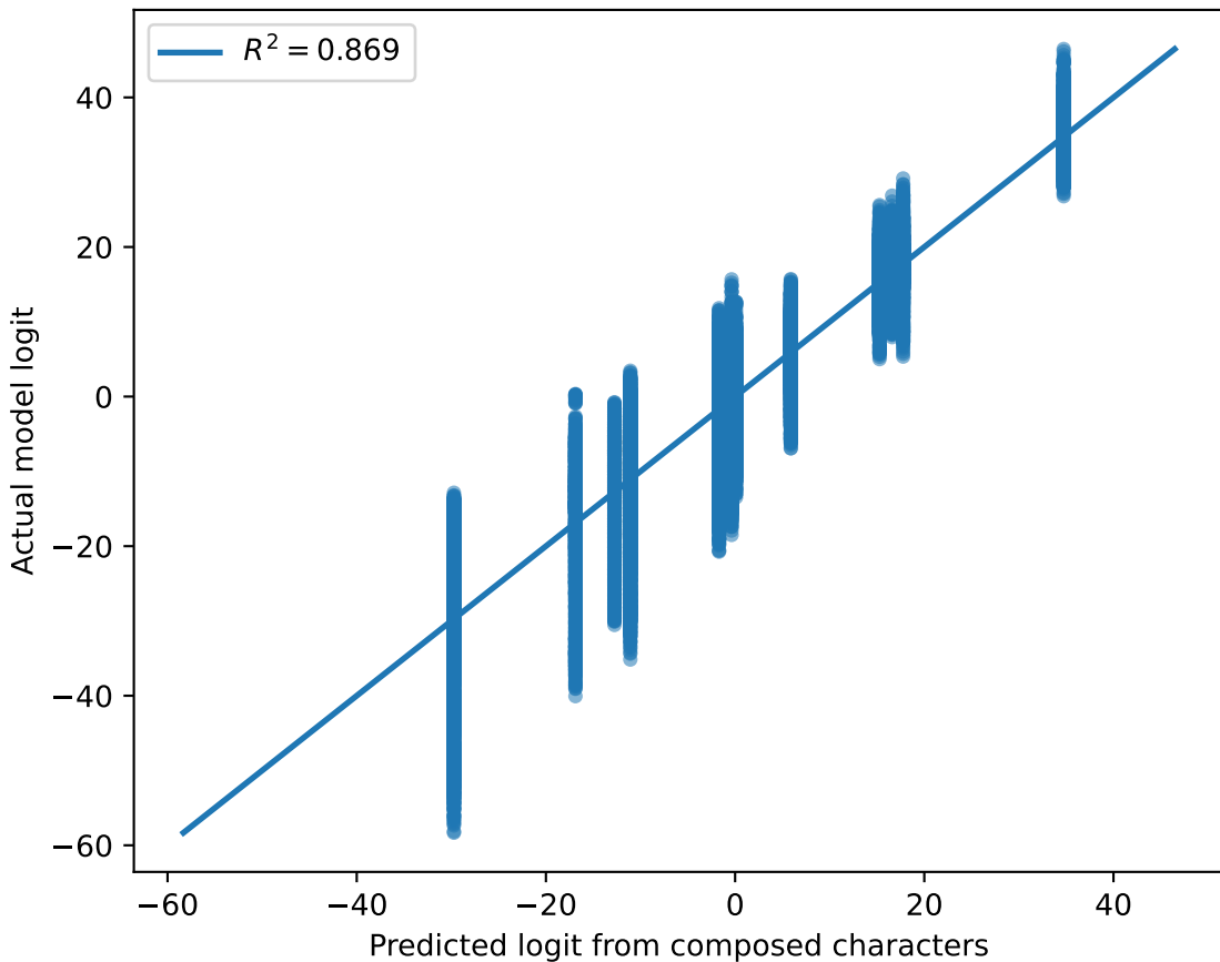
Character Logit Fit: J_5 \cong C_2 \times C_{10}
