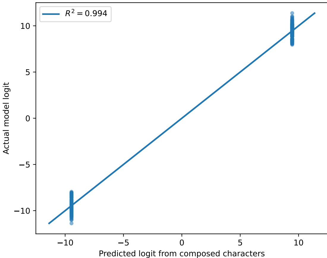
Character Logit Fit: J_{55} \cong C_2
