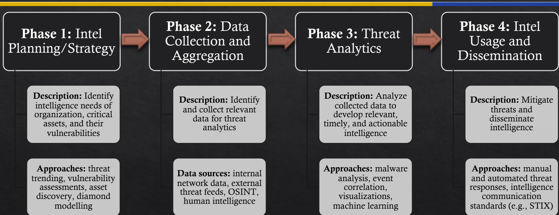
Four phased CTI Lifecycle
