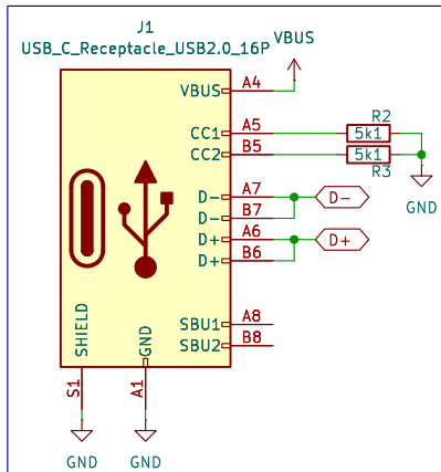
USB connector
