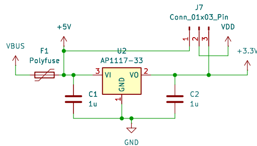
3.3 V regulator
