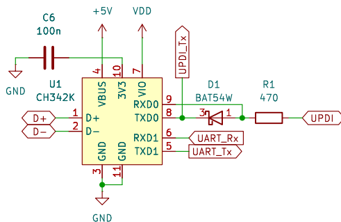
Dual UART and UPDI conversion
