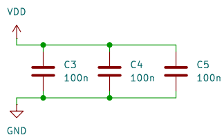
Bypass capacitors
