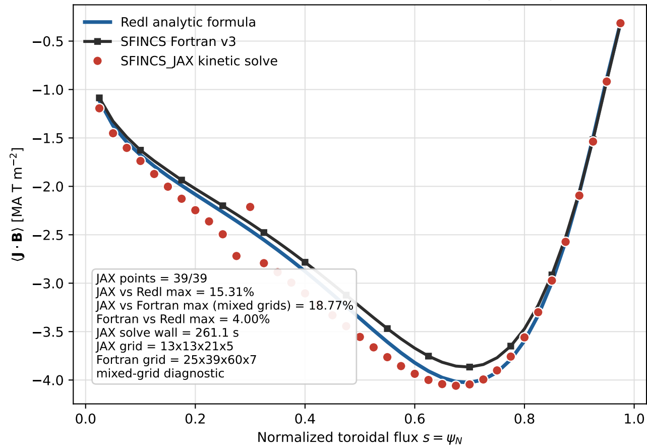
Quasi-helical benchmark (whole-radius mixed-grid diagnostic)
