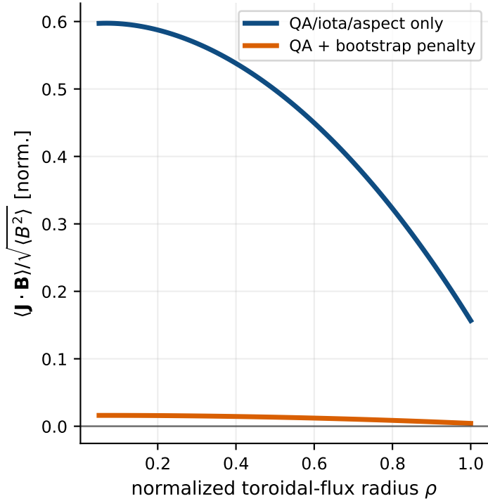
D. Bootstrap-current proxy profile
