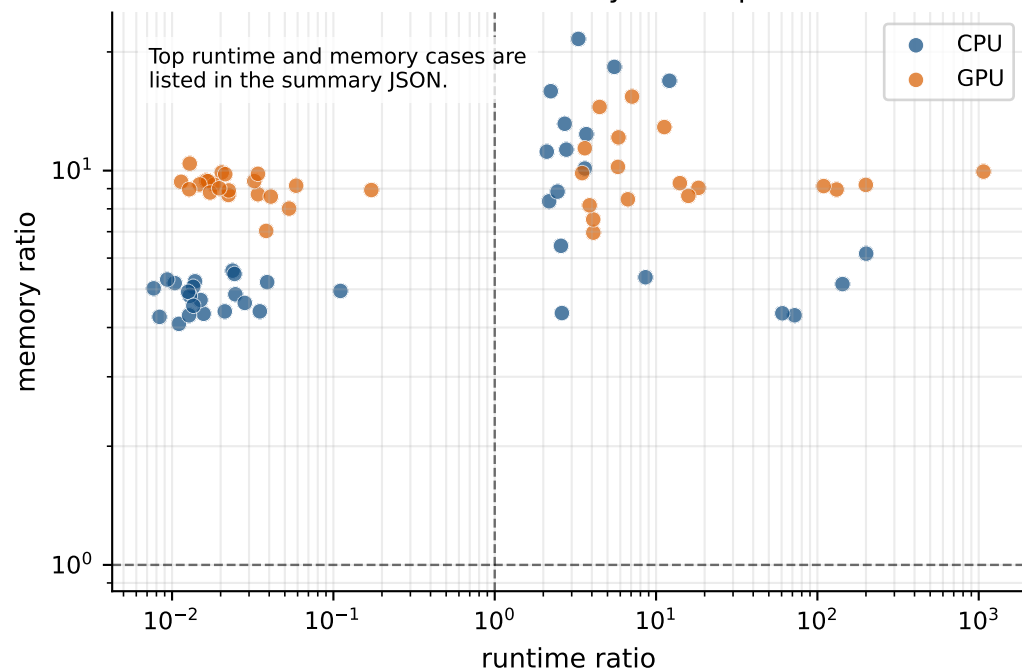
D. Runtime-memory trade space
