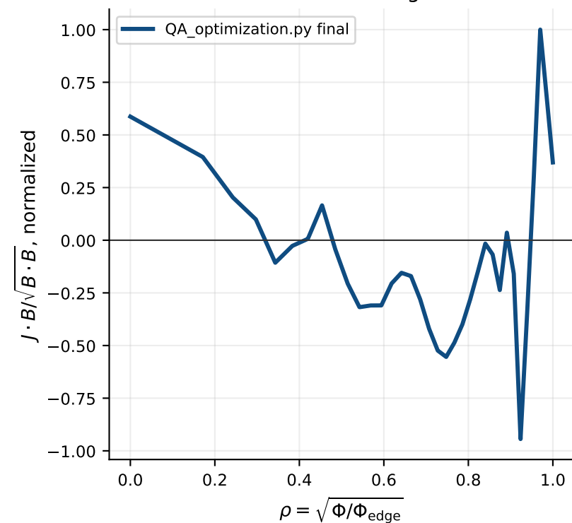
E. VMEC current diagnostic
