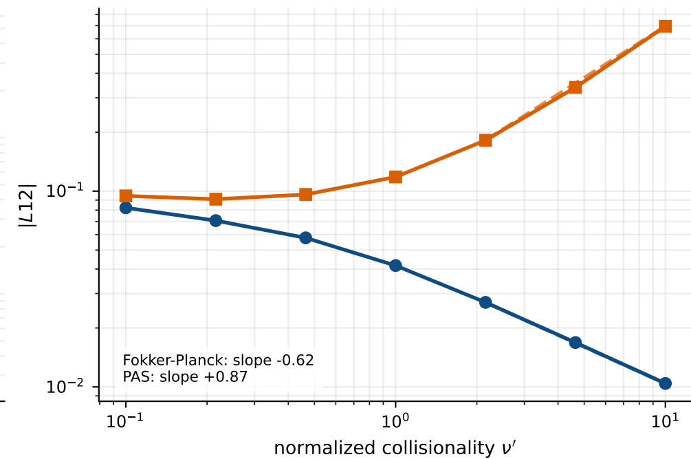
W7-X L12
