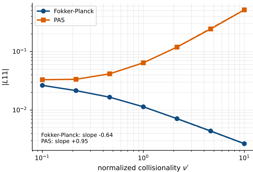
W7-X L11
