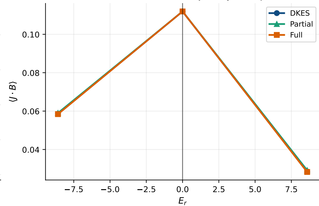
D. Stellarator-like trajectory sweep
