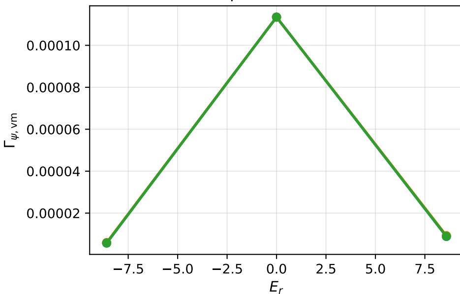
Stellarator-like trajectory-model sweep versus radial electric field (fast branch particle flux
