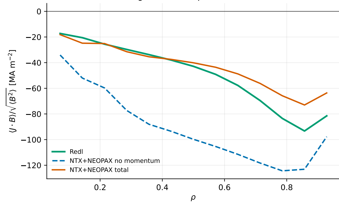
(c) Same-grid bootstrap-current observable
