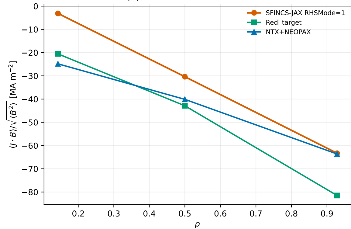
(a) Profile-current observable
