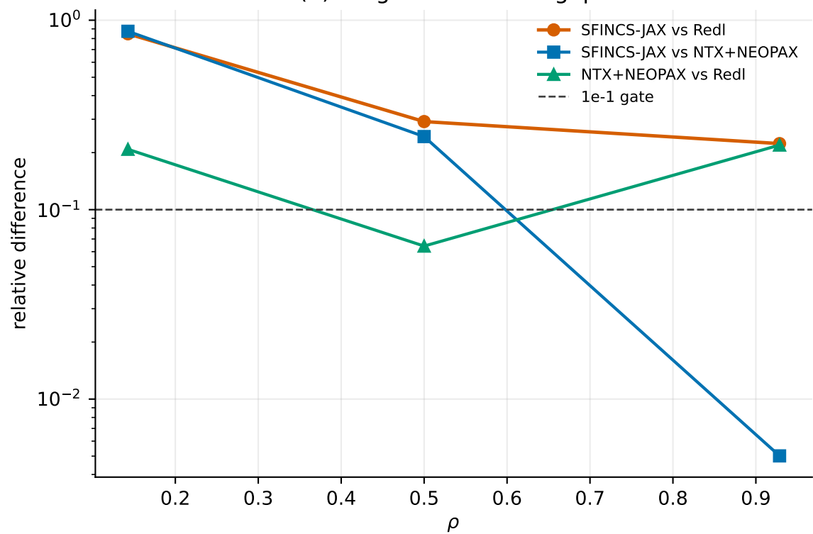
(b) Diagnostic current gaps
