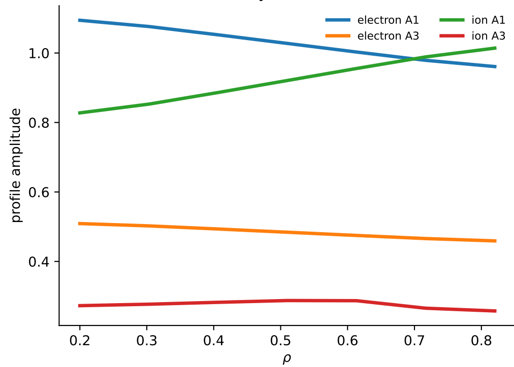
Final Thermodynamic-Force Profiles
