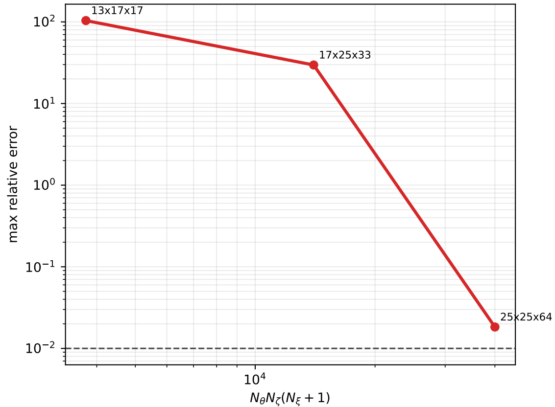
Bootstrap-current convergence
