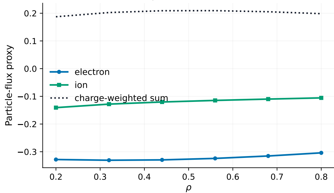
Ambipolar residual closure
