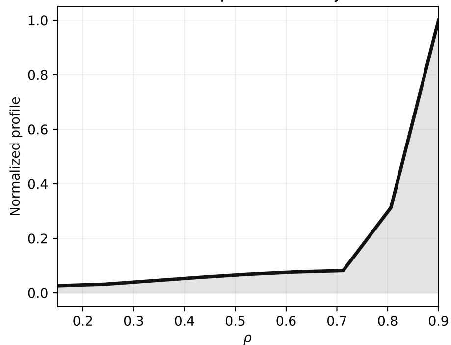
Bootstrap-Current Proxy
