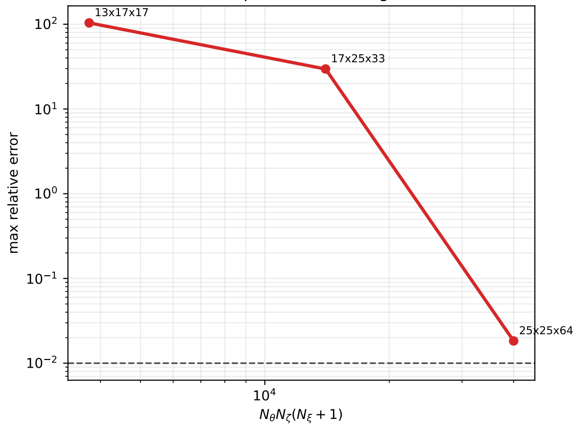
Bootstrap-current convergence
